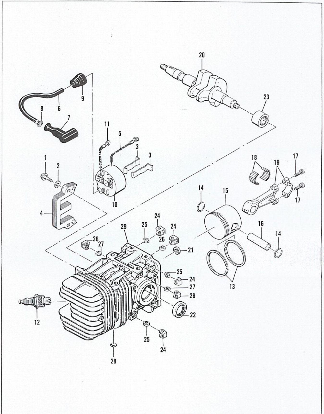
Figure 6. Powerhead
