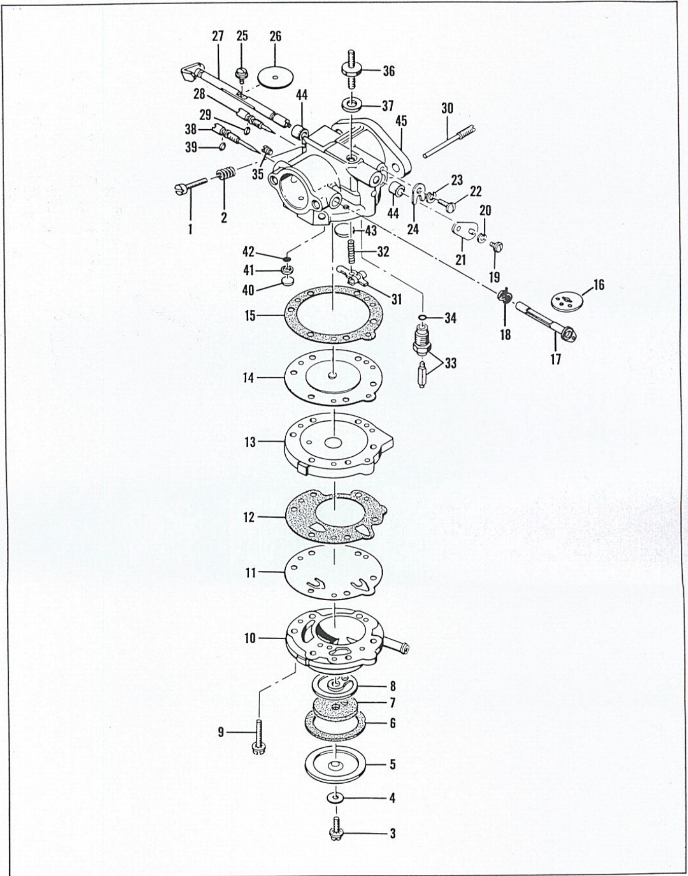
Figure 5. Carburetor
