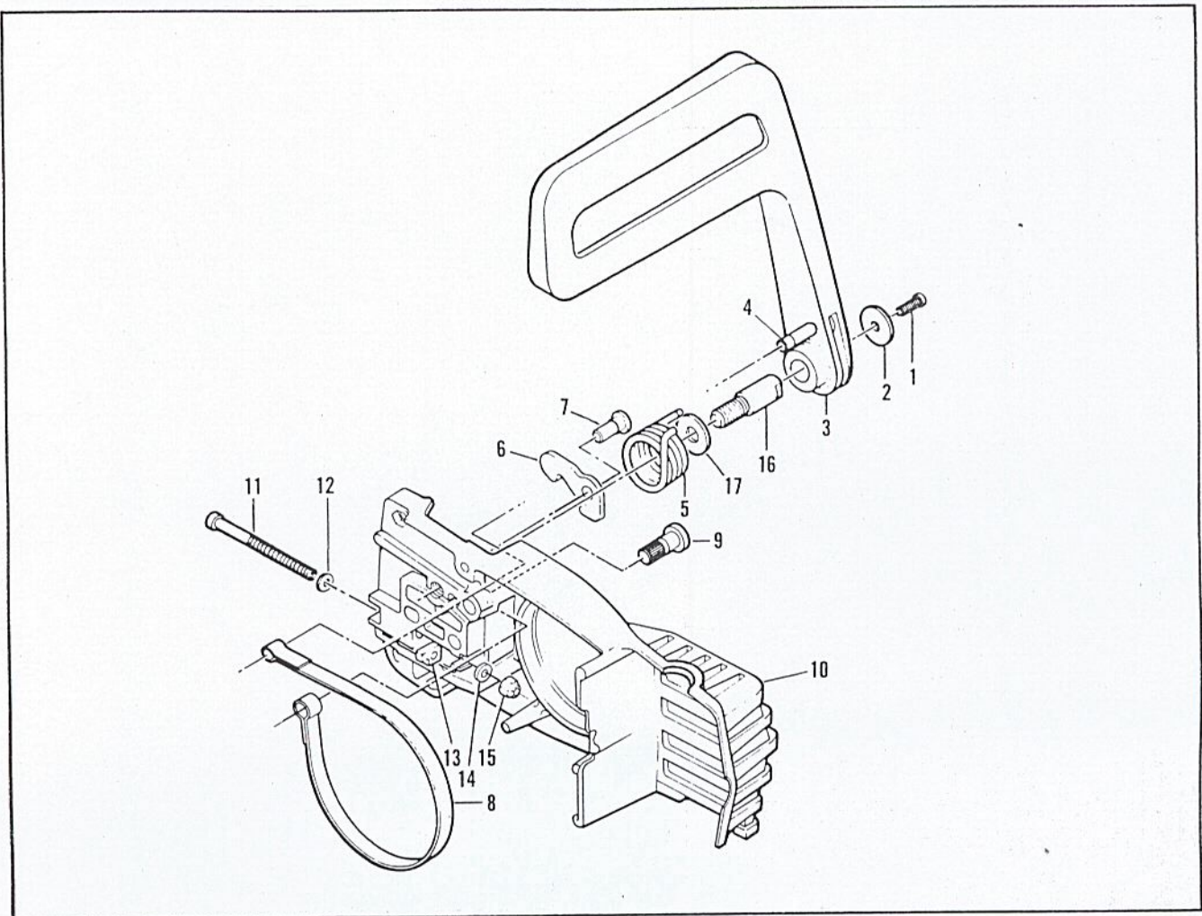
Figure 3 CHAIN BRAKE® ASSEMBLY
