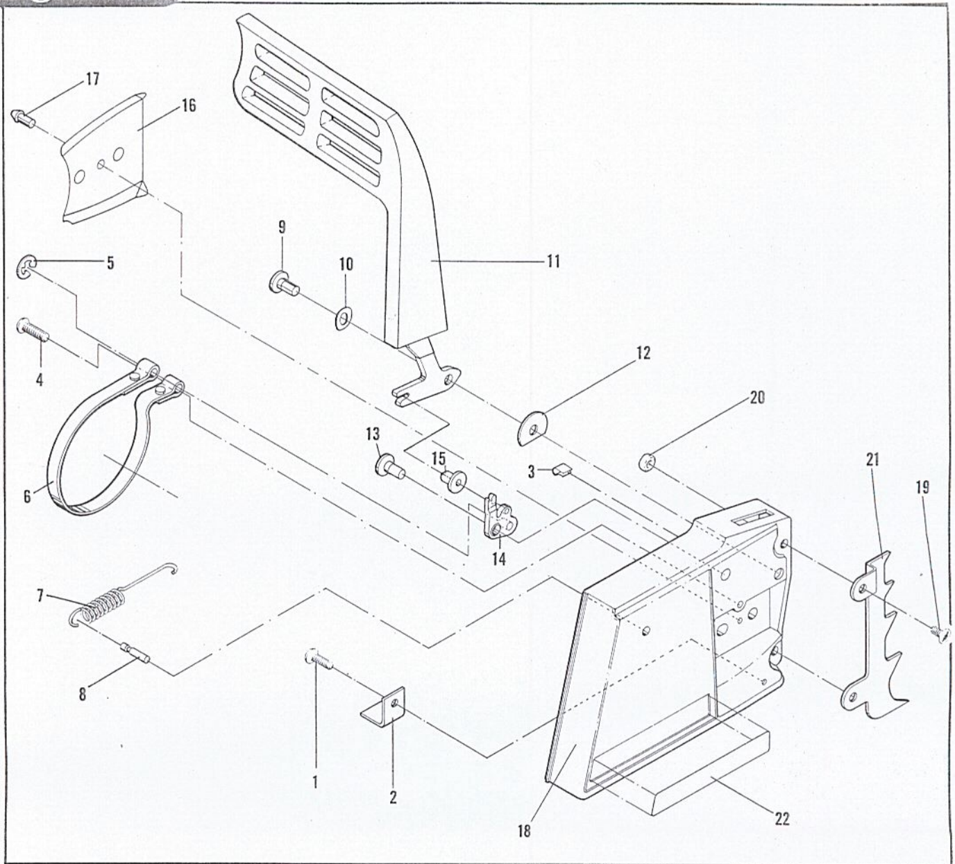
Figure 3 CHAIN BRAKE ASSEMBLY
