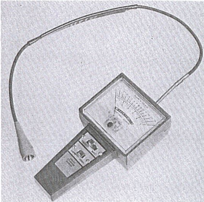
TACHOMETER (2 & 4 cycle, 0–15,000 rpm) PART NO. 91424 MODELS: All
