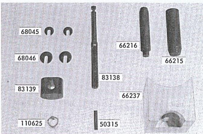
KIT - BLIND PISTON PART NO. 83207 MODELS: MC 101-101C
