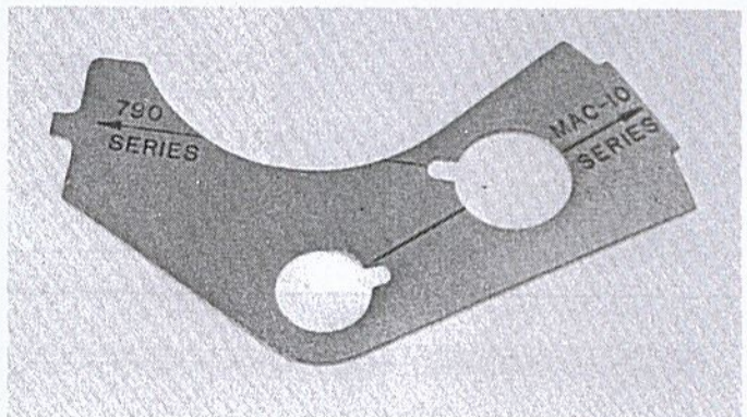
TIMING GUIDE PART NO. 86419 MODELS: Combination 10 Series, 250, PM60, SP 125 (26° BTDC timing), 790 Series
