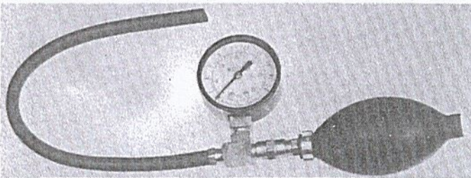
PRESSURE TEST TOOL PART NO. 90533
