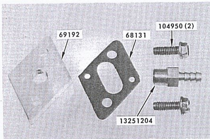
KIT - PRESSURE TESTING PART NO. 69191 MODELS: MAC 10 Series w/ SDC Carburetor, PM 55, PM 60, 7-10A, CP 55, CP 70, SP 60, SP 80, SP 81, SP 105, SP 125C
