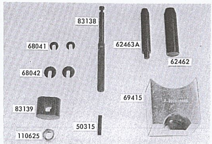
KIT - BLIND PISTON PART NO. 83209 MODELS: S797, CP 125, CP 125S, MC 101A, MC 101AA (SP 105, PM 105, SP 125C, 895C requires Bearing Driver 63095 in Kit 84453)
