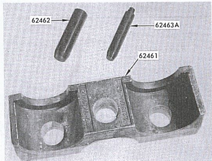
KIT - PISTON TOOL PART NO. 62459A MODELS: Use with all McCulloch 2.165, 2.218, and 2.125" diameter pistons, including 0.030" oversize
