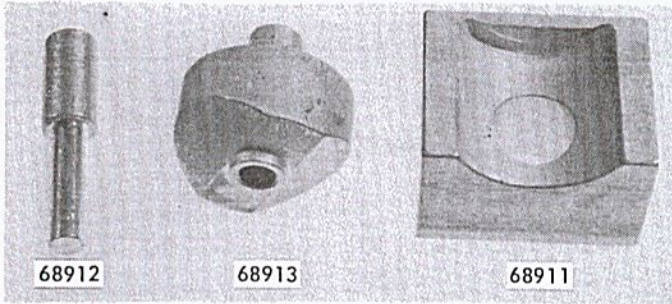
KIT - PISTON TOOL PART NO. 68915 MODELS: PM6A, MM35 (2.0 cu. in.)
