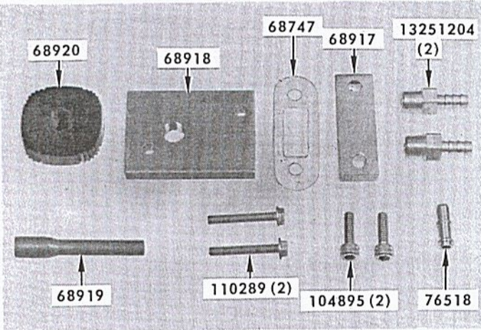
KIT - PRESSURE TESTING PART NO. 68916 MODELS: PM6A, MM Series
