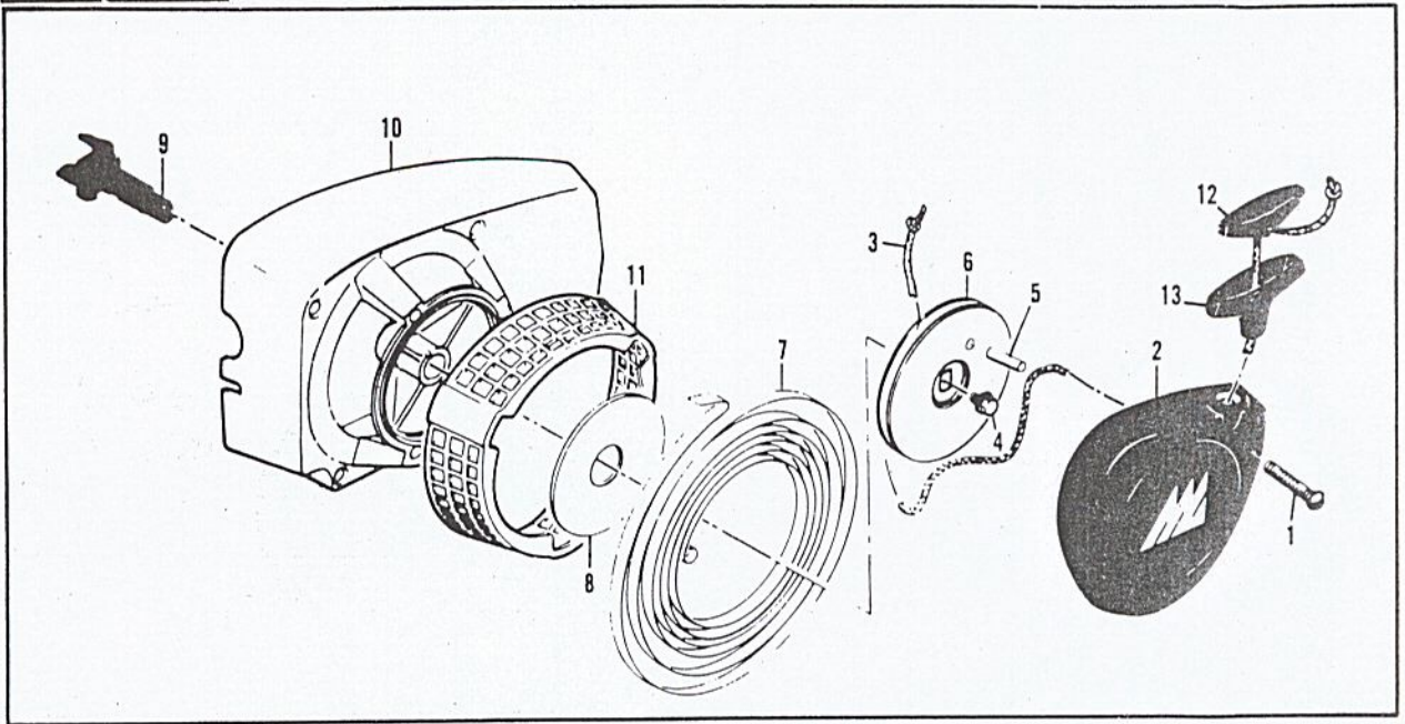
FIGURE 6 FAN HOUSING & STARTER ASSEMBLY
