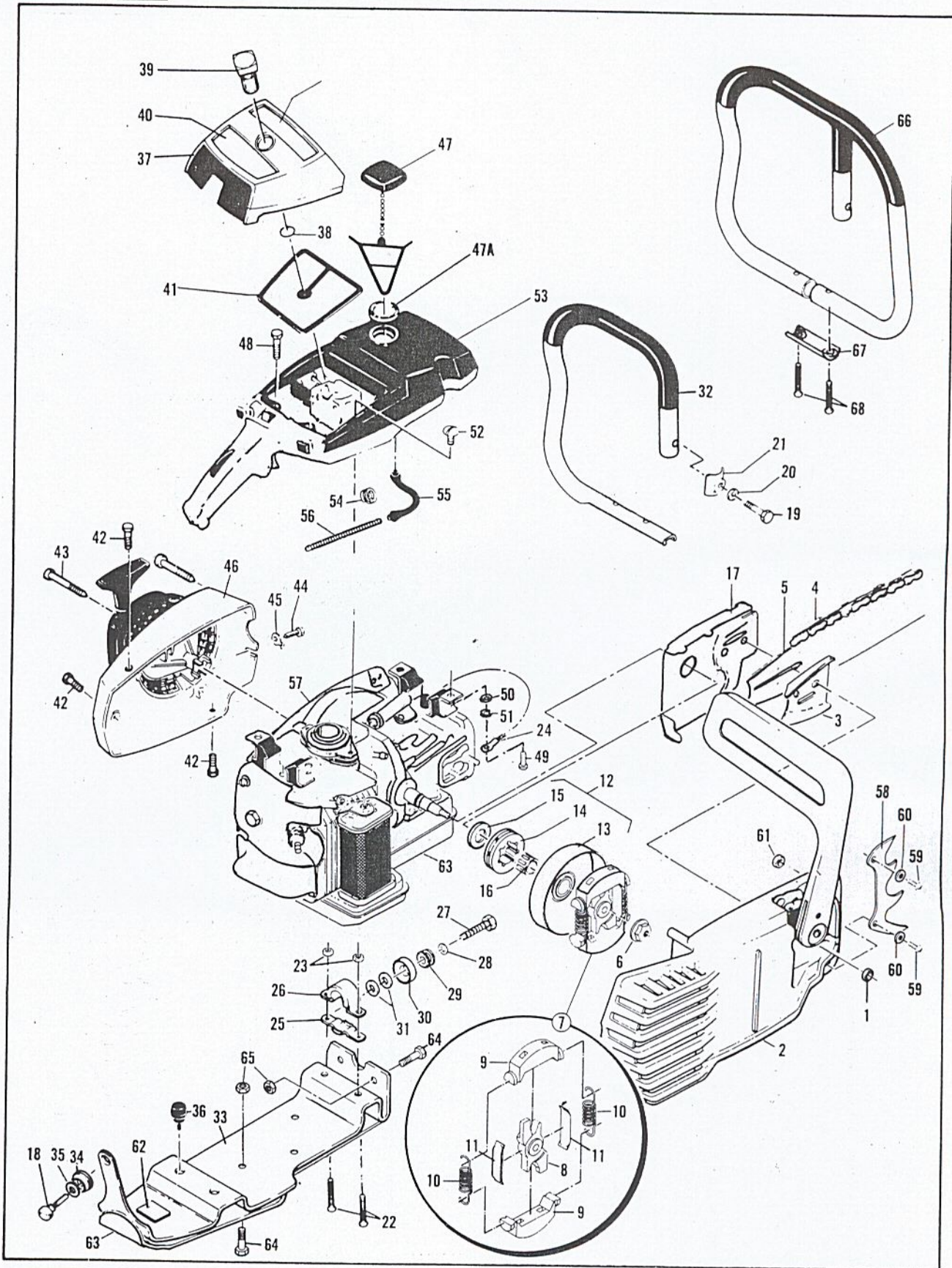
FIGURE 1 GENERAL ASSEMBLY
