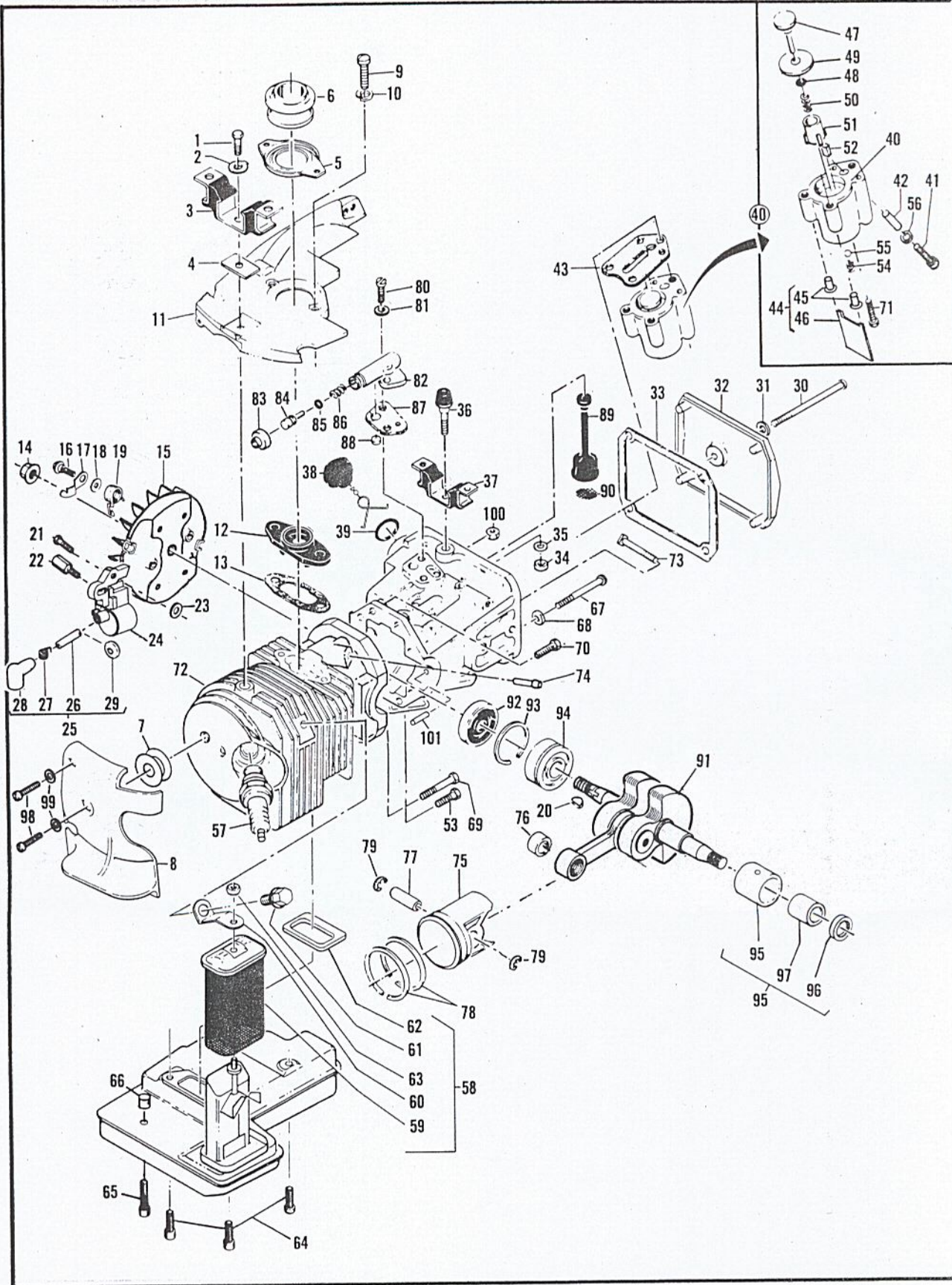
FIGURE 3 POWERHEAD ASSEMBLY
