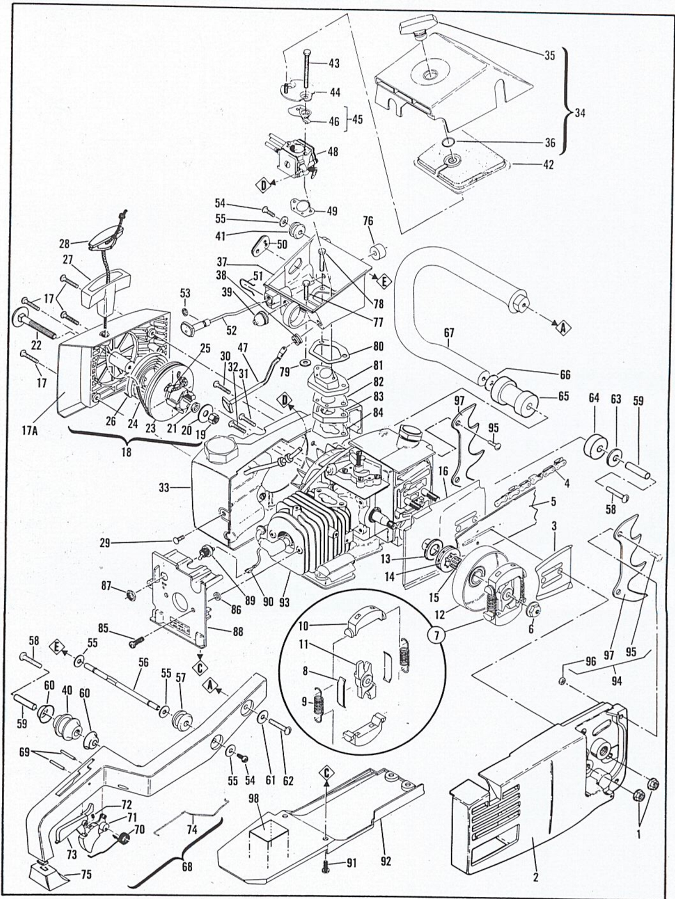
Figure 1 GENERAL ASSEMBLY
