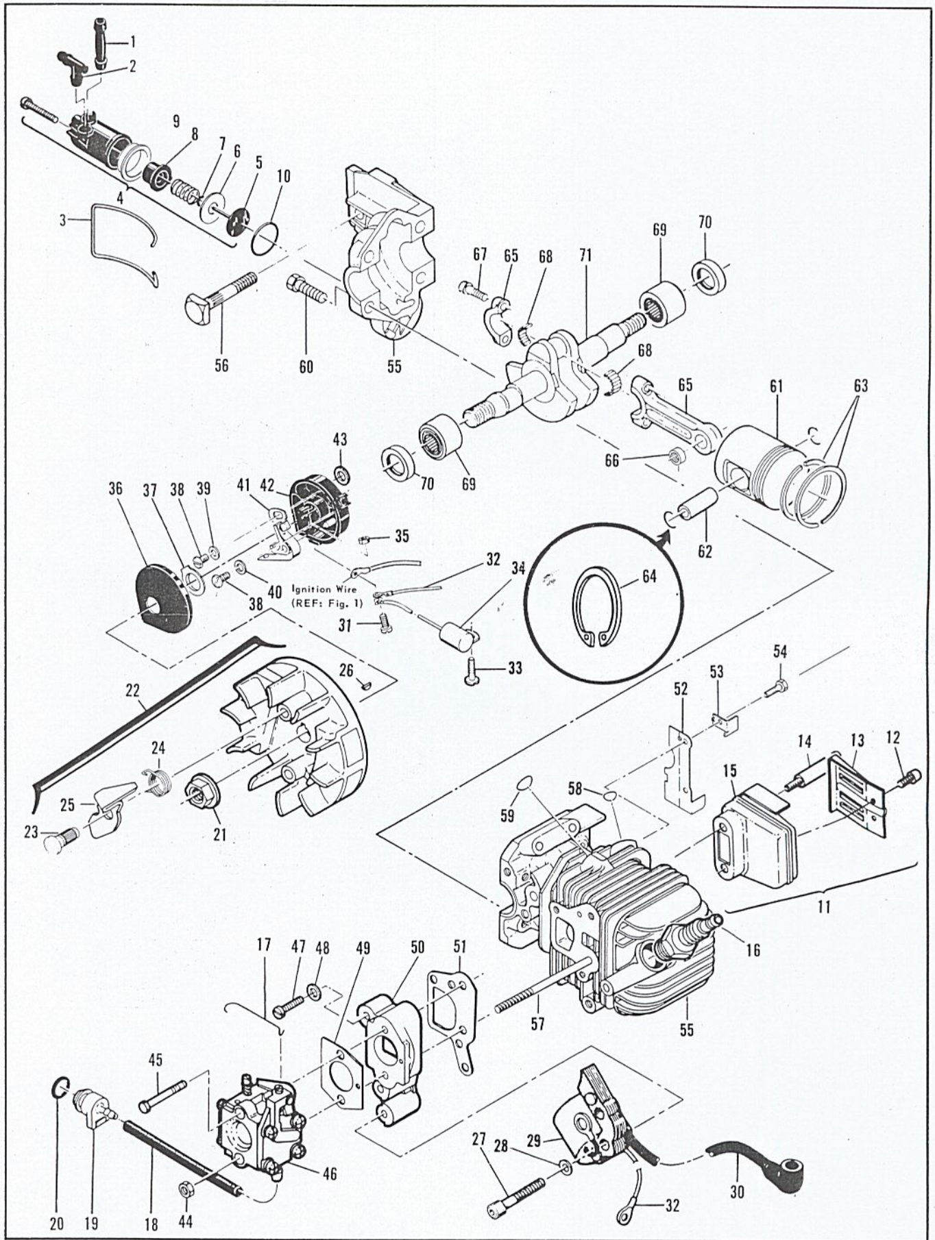
Figure 5. Powerhead Assembly
