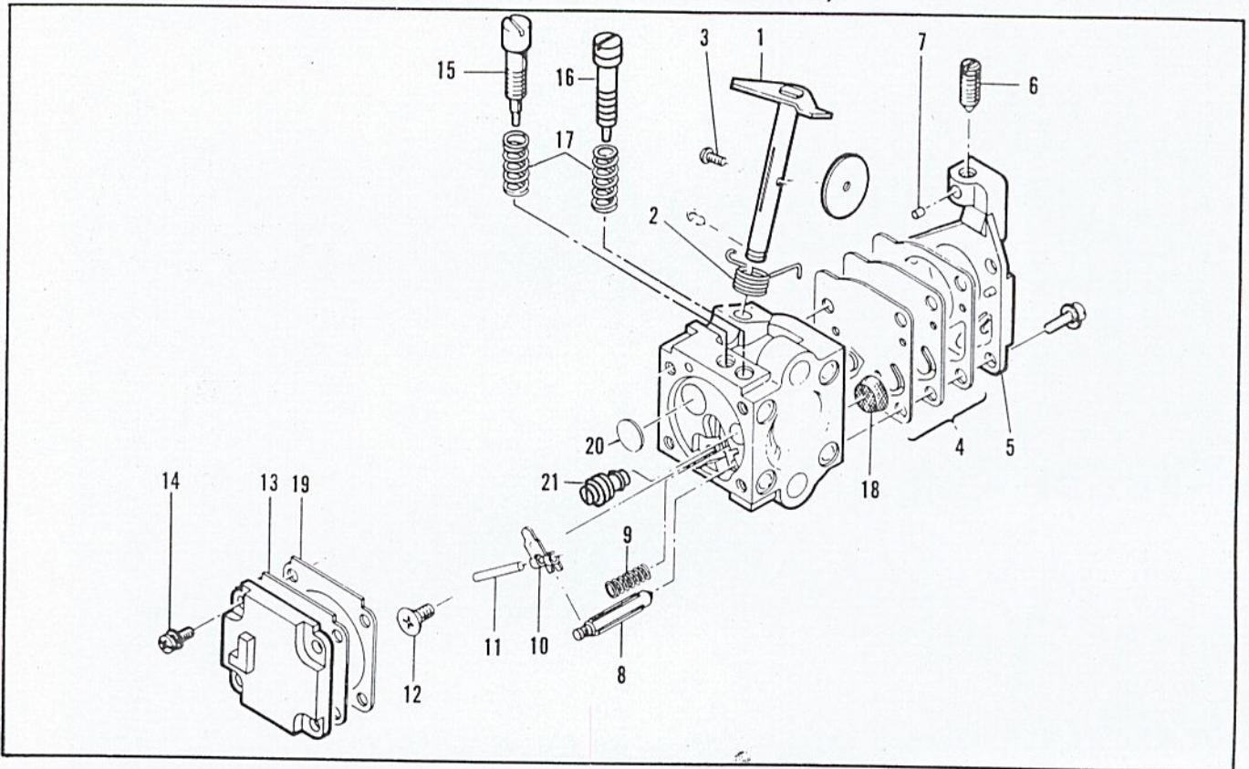
Figure 6. Carburetor Assembly
