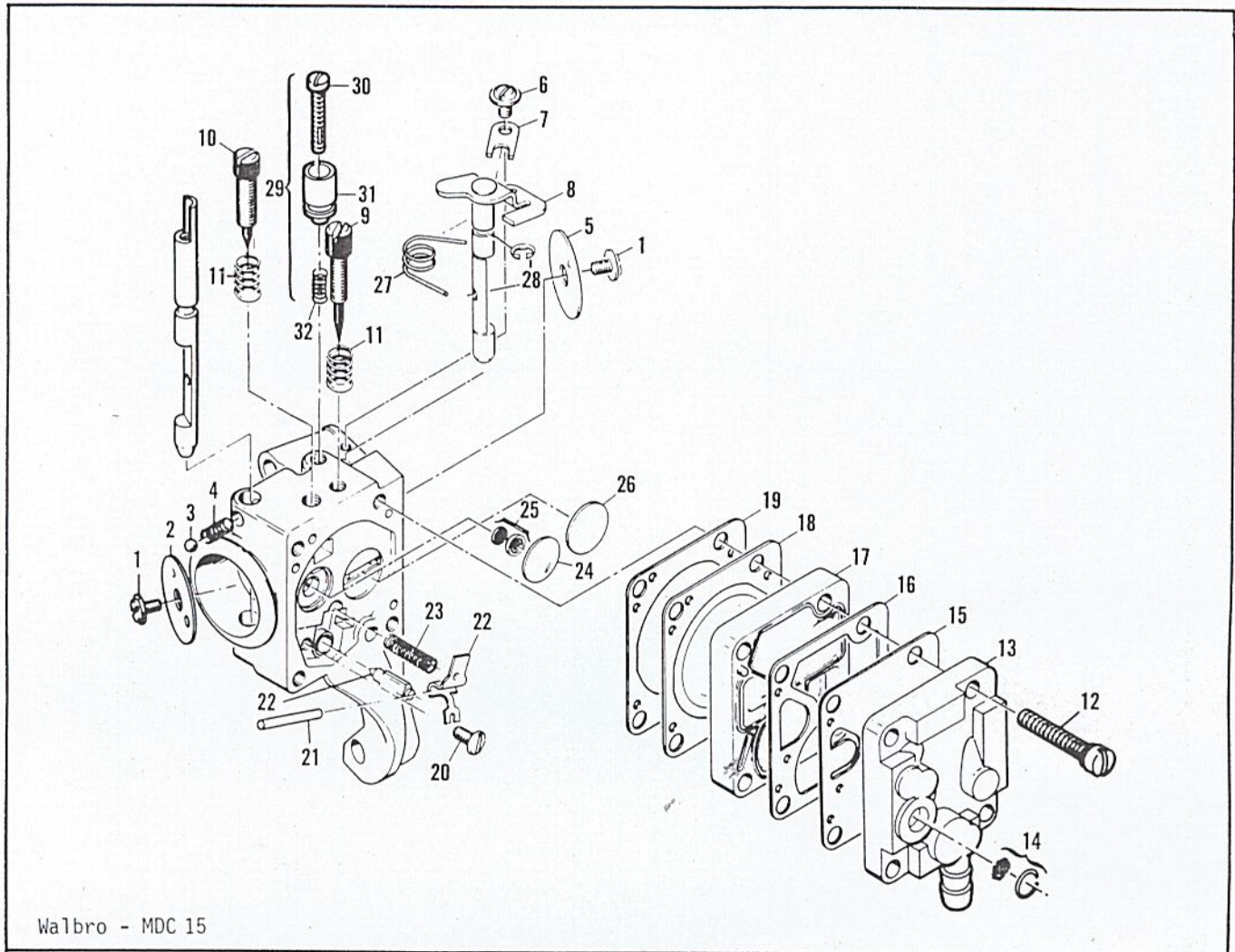
Figure 2. Carburetor Assembly
