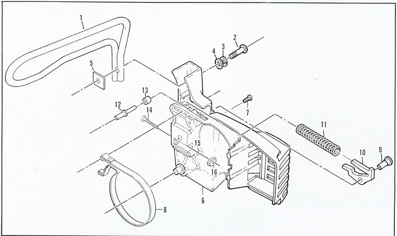
Figure 5. CHAIN BRAKE Assembly
