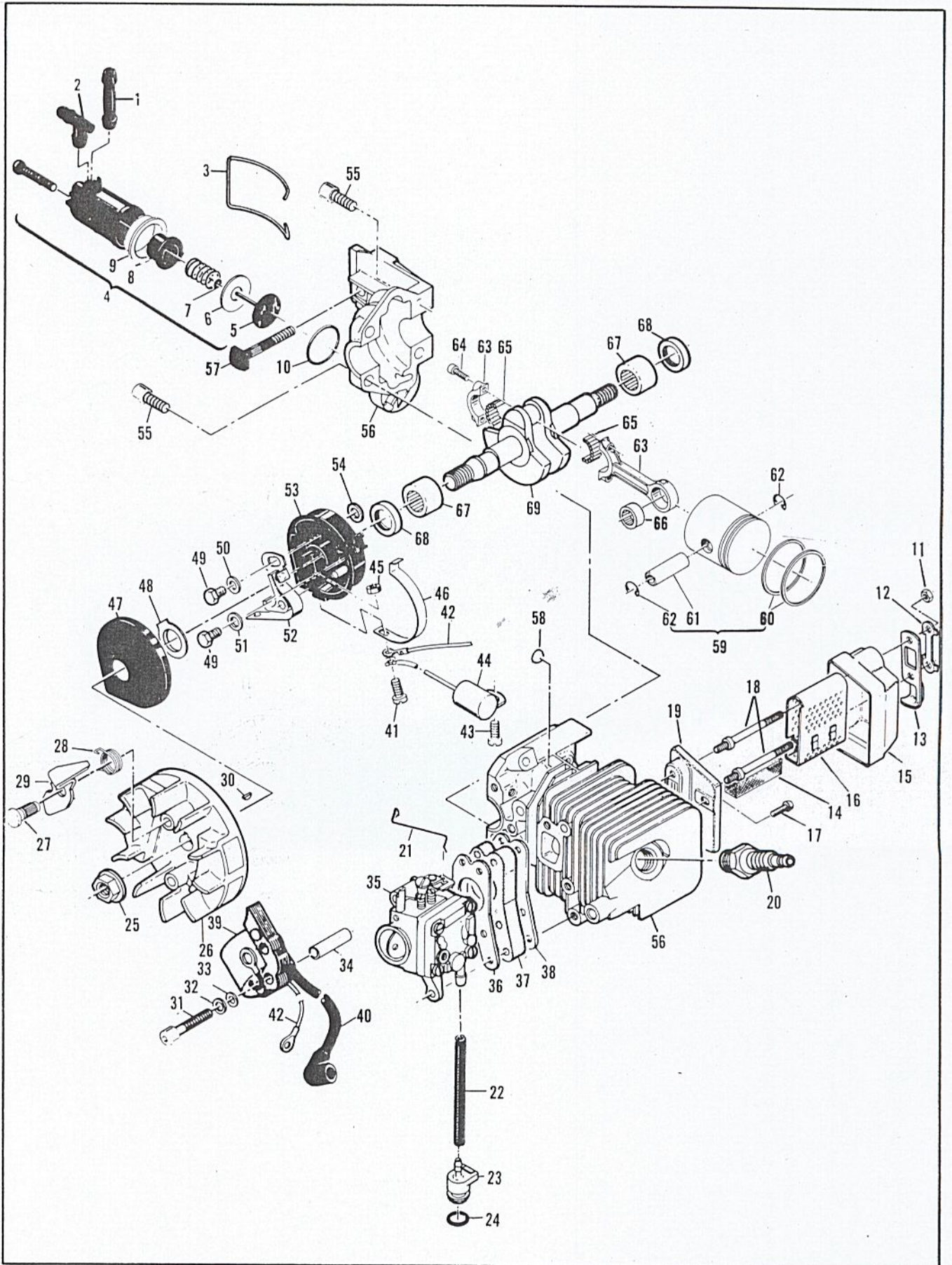
Figure 4. Powerhead Assembly.
