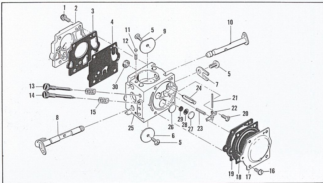
Figure 4. Carburetor Assembly
