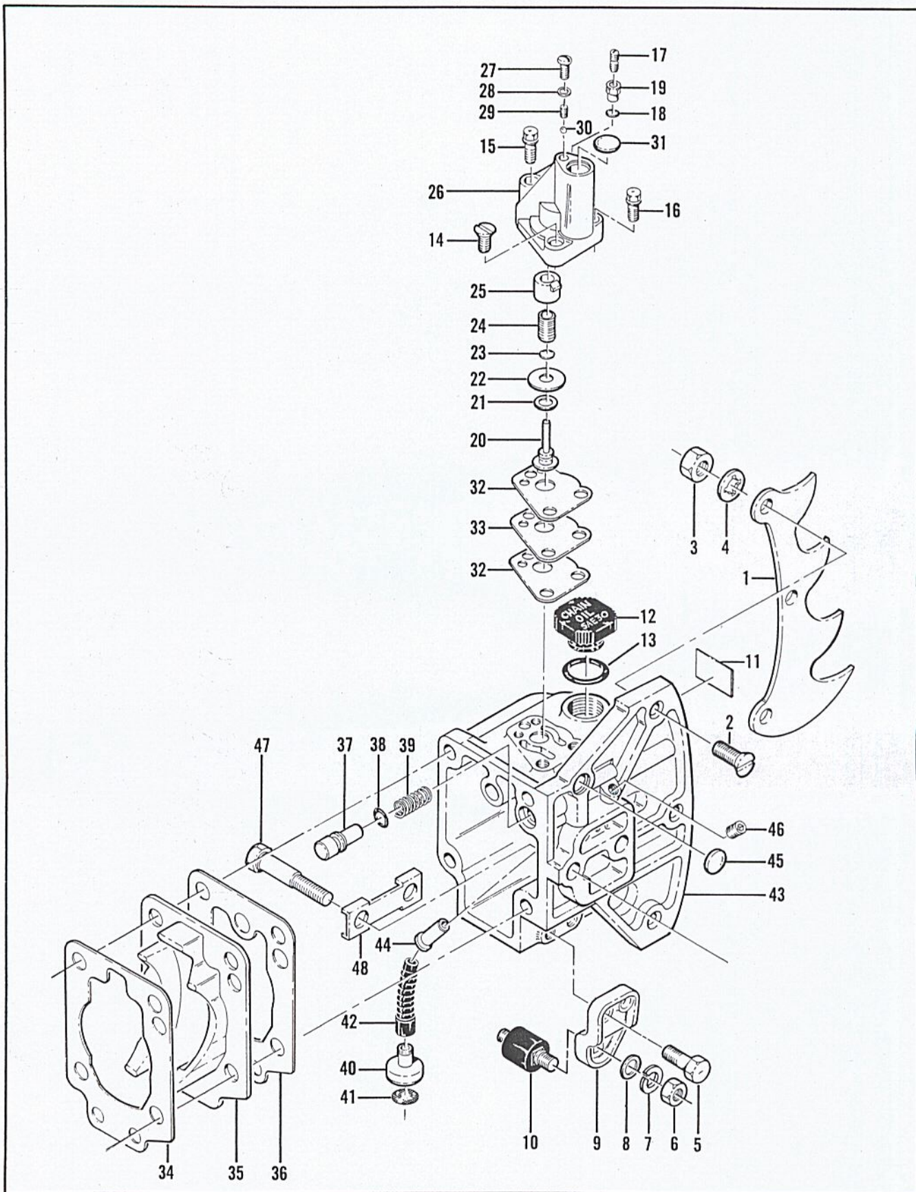
Figure 6. Oiler Tank and Pump Assemblies
