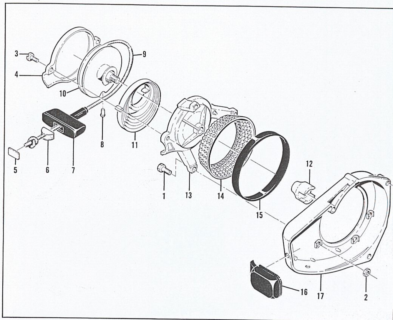
FIGURE 3. FAN HOUSING AND STARTER ASSEMBLY
