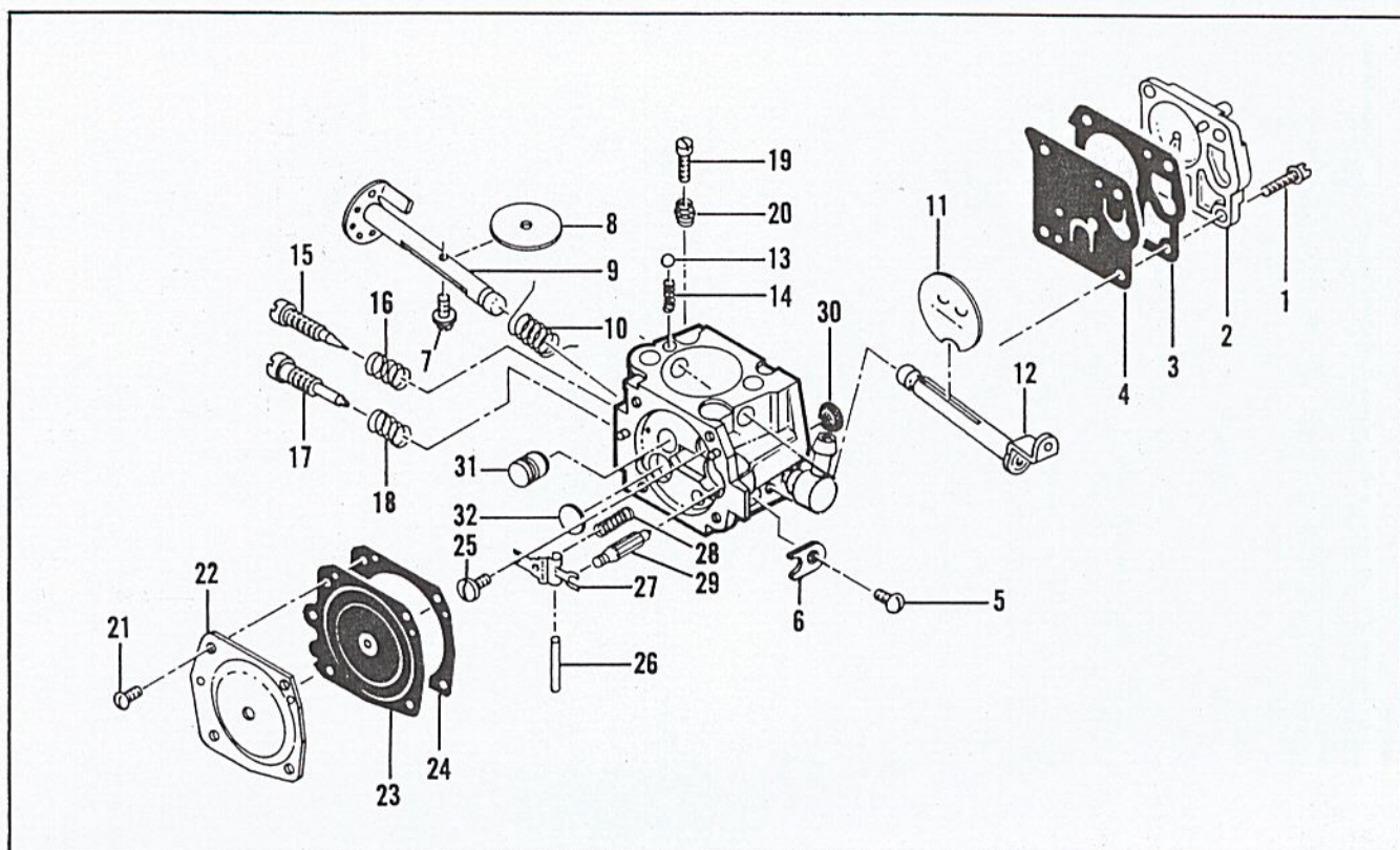
Figure 5A. Tillotson Carburetor Assembly
