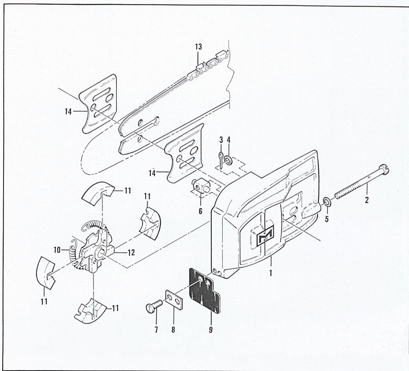
FIGURE 2. CLUTCH GUARD AND CLUTCH ASSEMBLIES
