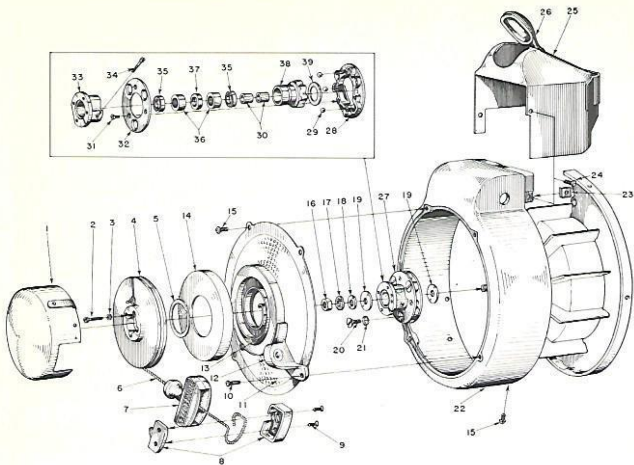
FIGURE 1 — RECOIL STARTER
