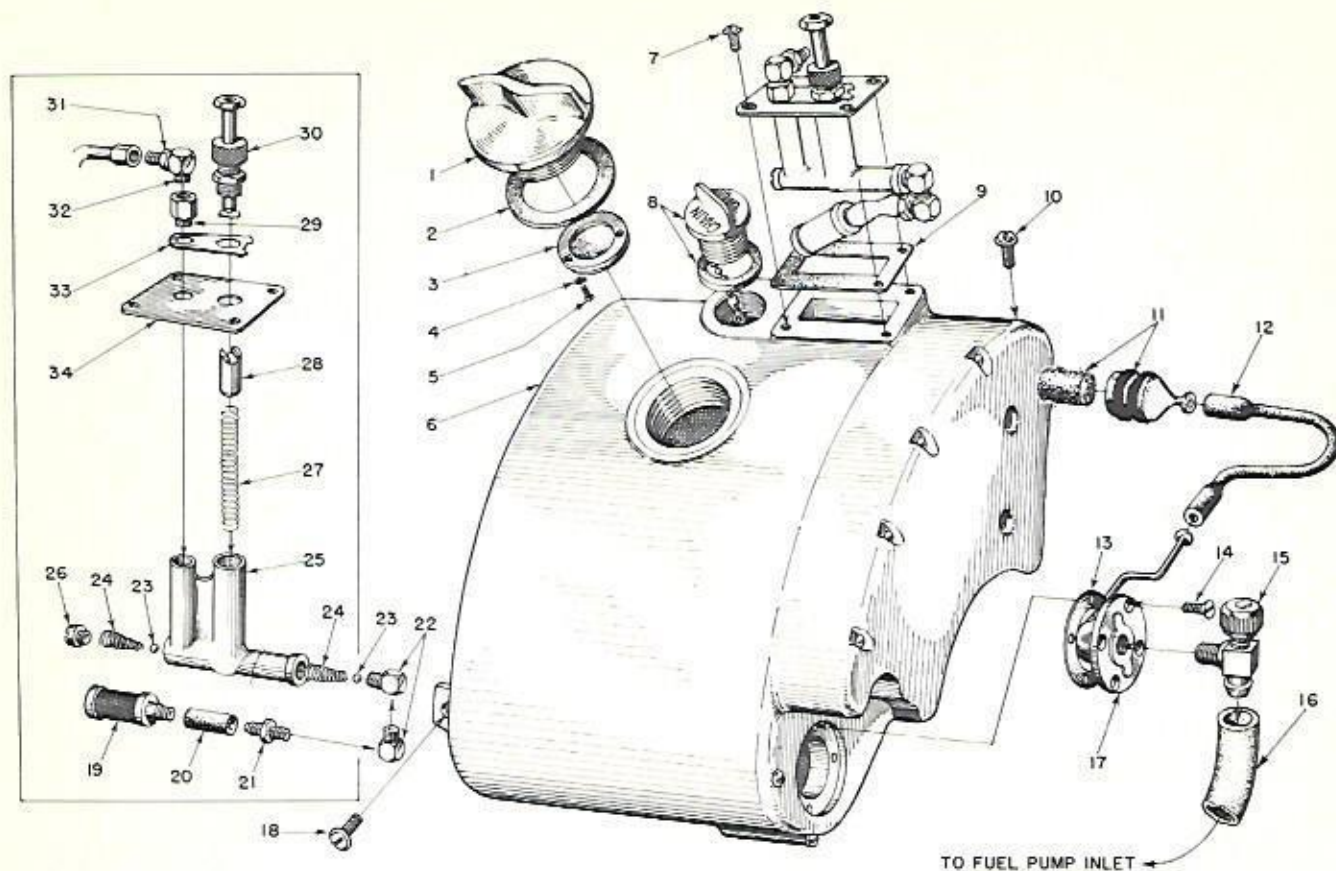
FIGURE 3 — FUEL TANK
