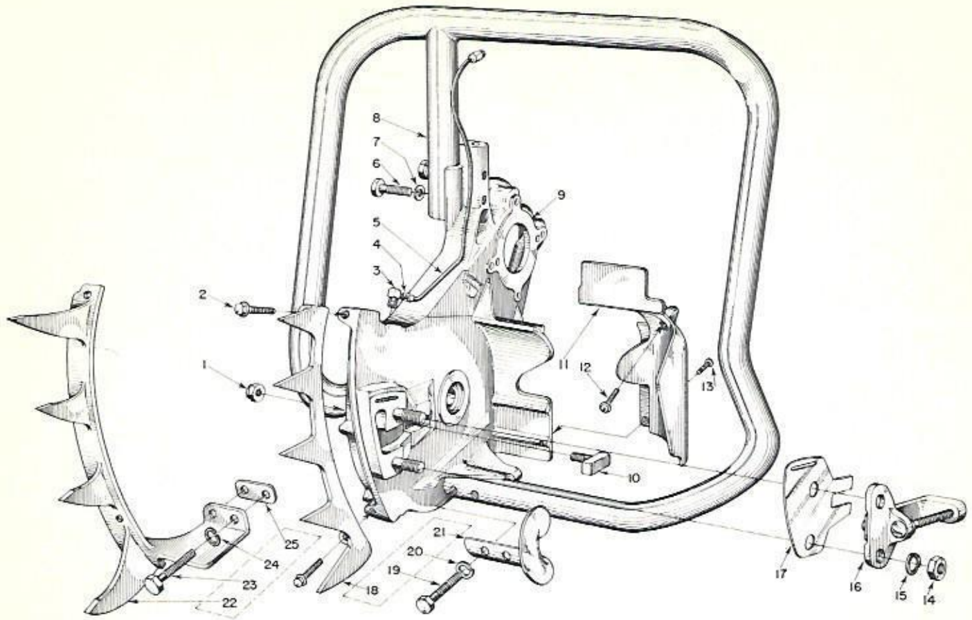
FIGURE 9 — SAW END GROUP
