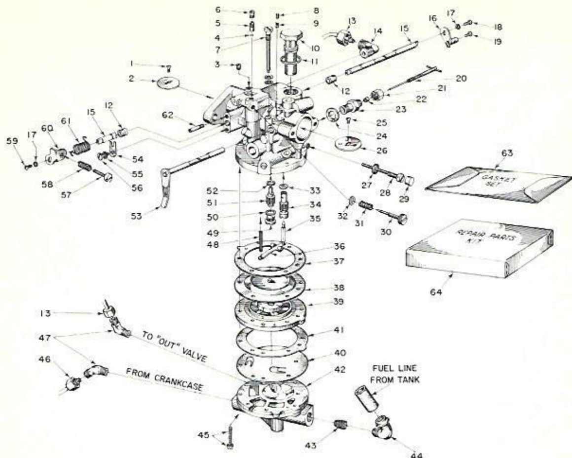
FIGURE 5 — TILLOTSON CARBURETOR PARTS
