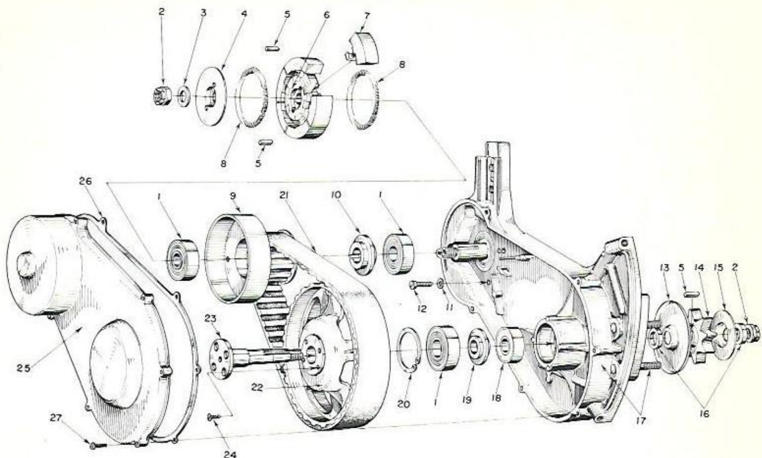
FIGURE 8 — DRIVE CASE
