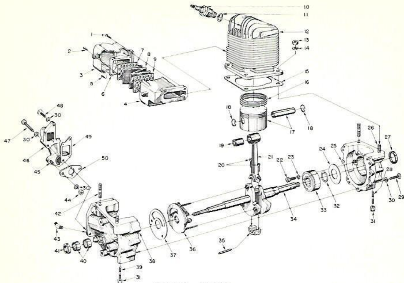
FIGURE 7 — ENGINE
