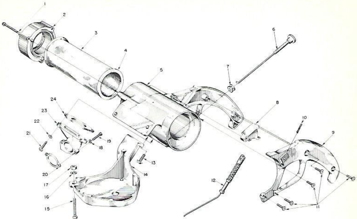
FIGURE 4 — PISTOL GRIP
