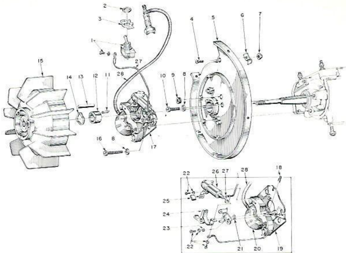
FIGURE 2 — IGNITION
