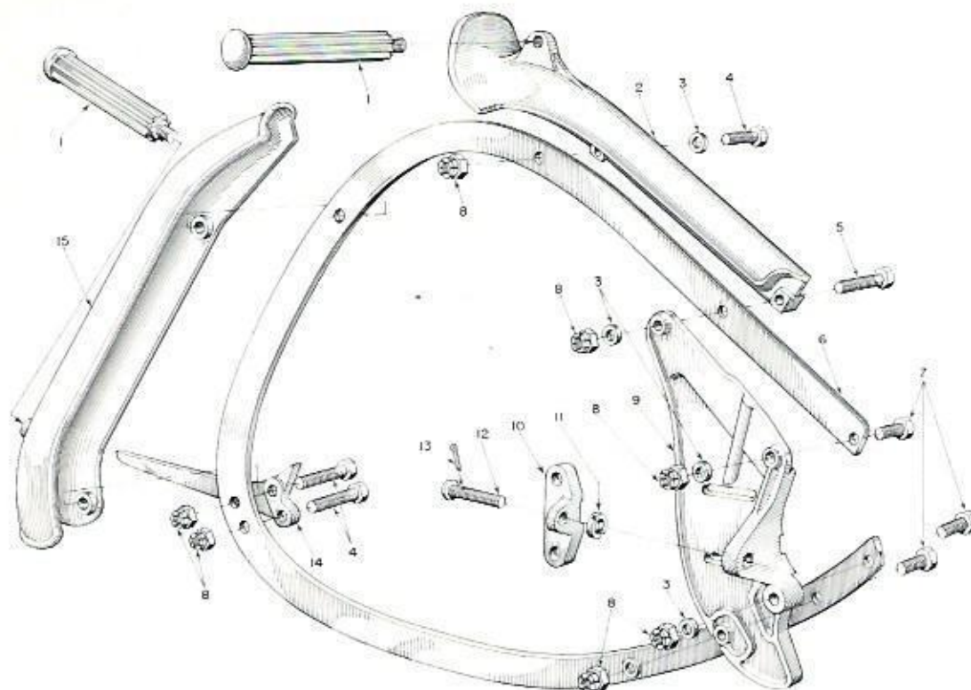
FIGURE 11 — BOW PARTS
