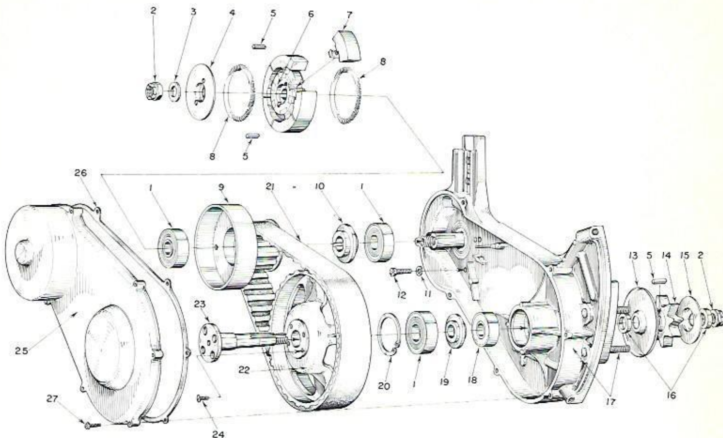
FIGURE 8 — DRIVE CASE
