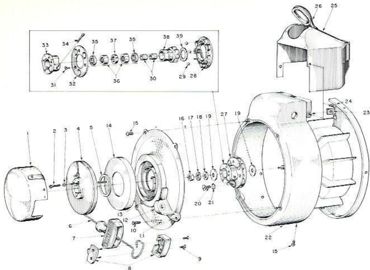
FIGURE 1 — RECOIL STARTER
