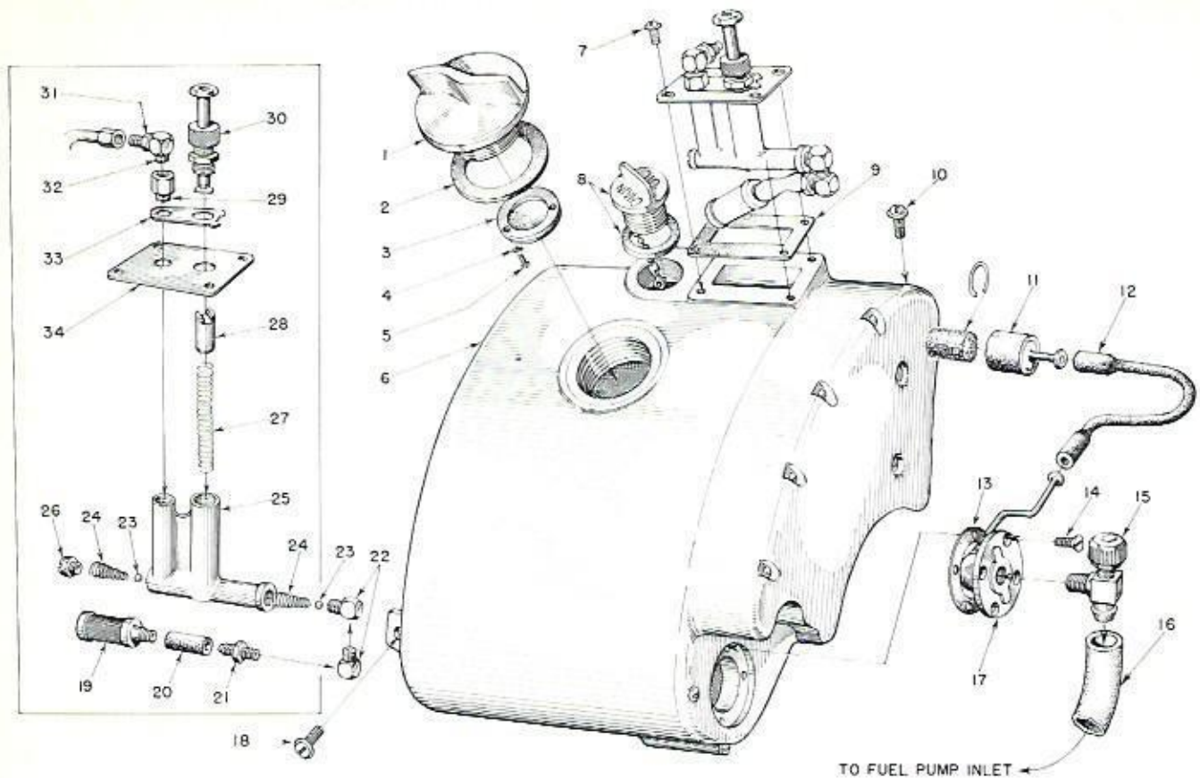
FIGURE 3 — FUEL TANK
