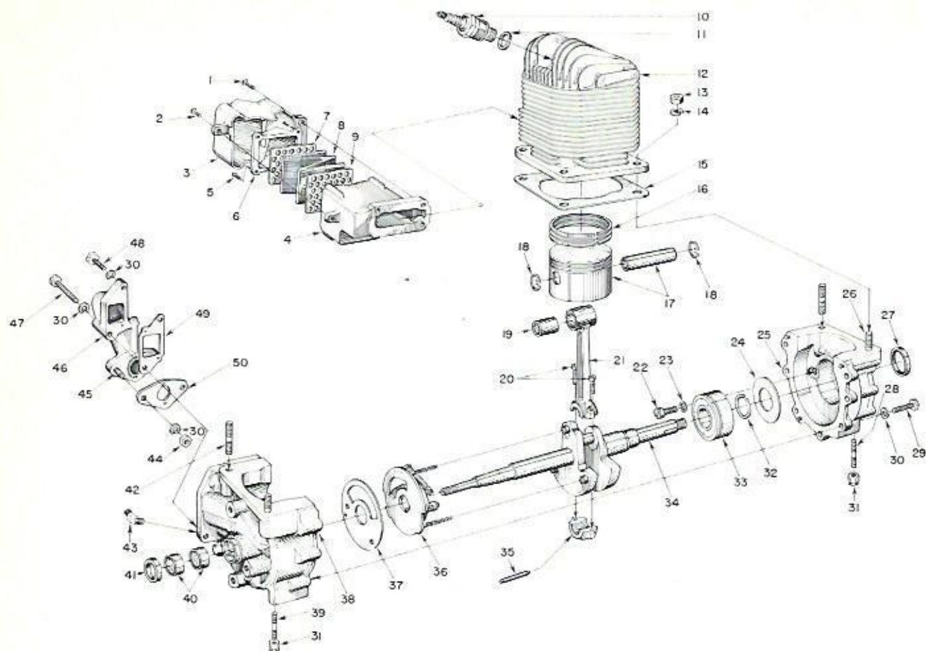
FIGURE 7 — ENGINE
