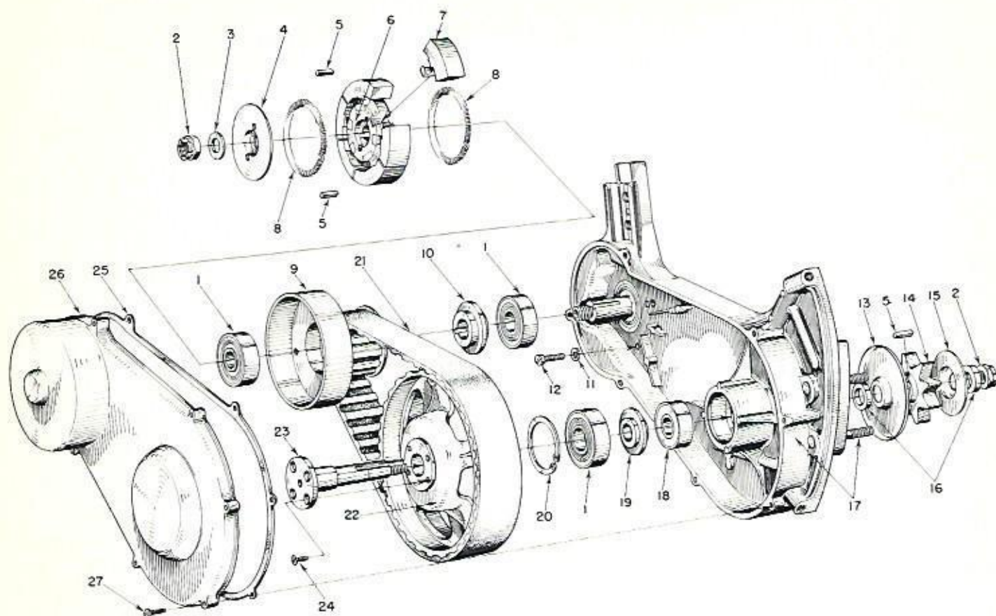
FIGURE 7—DRIVE CASE PARTS
