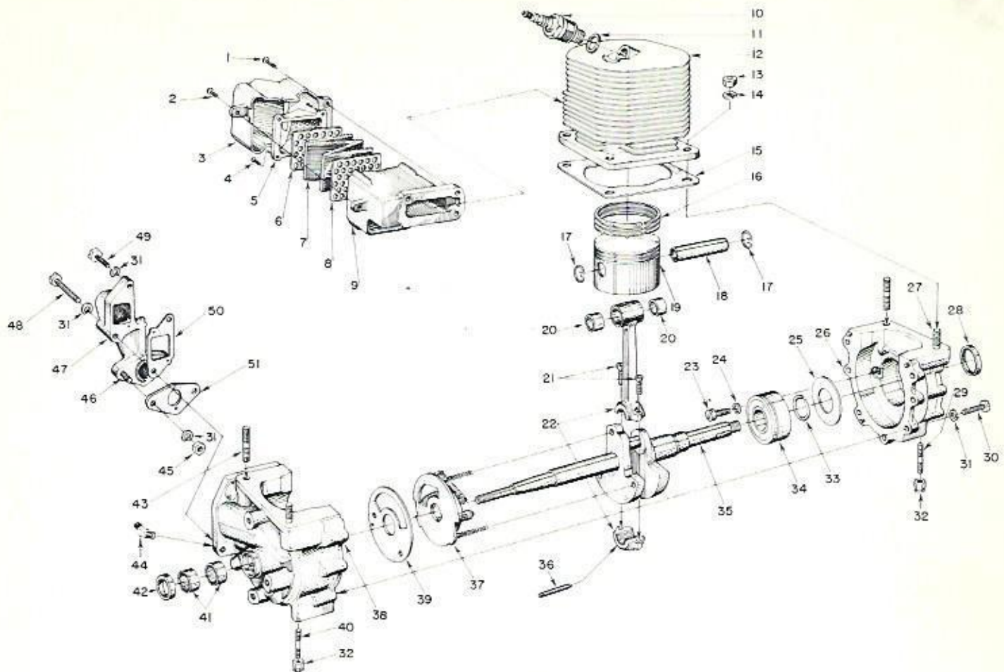
FIGURE 6—ENGINE PARTS
