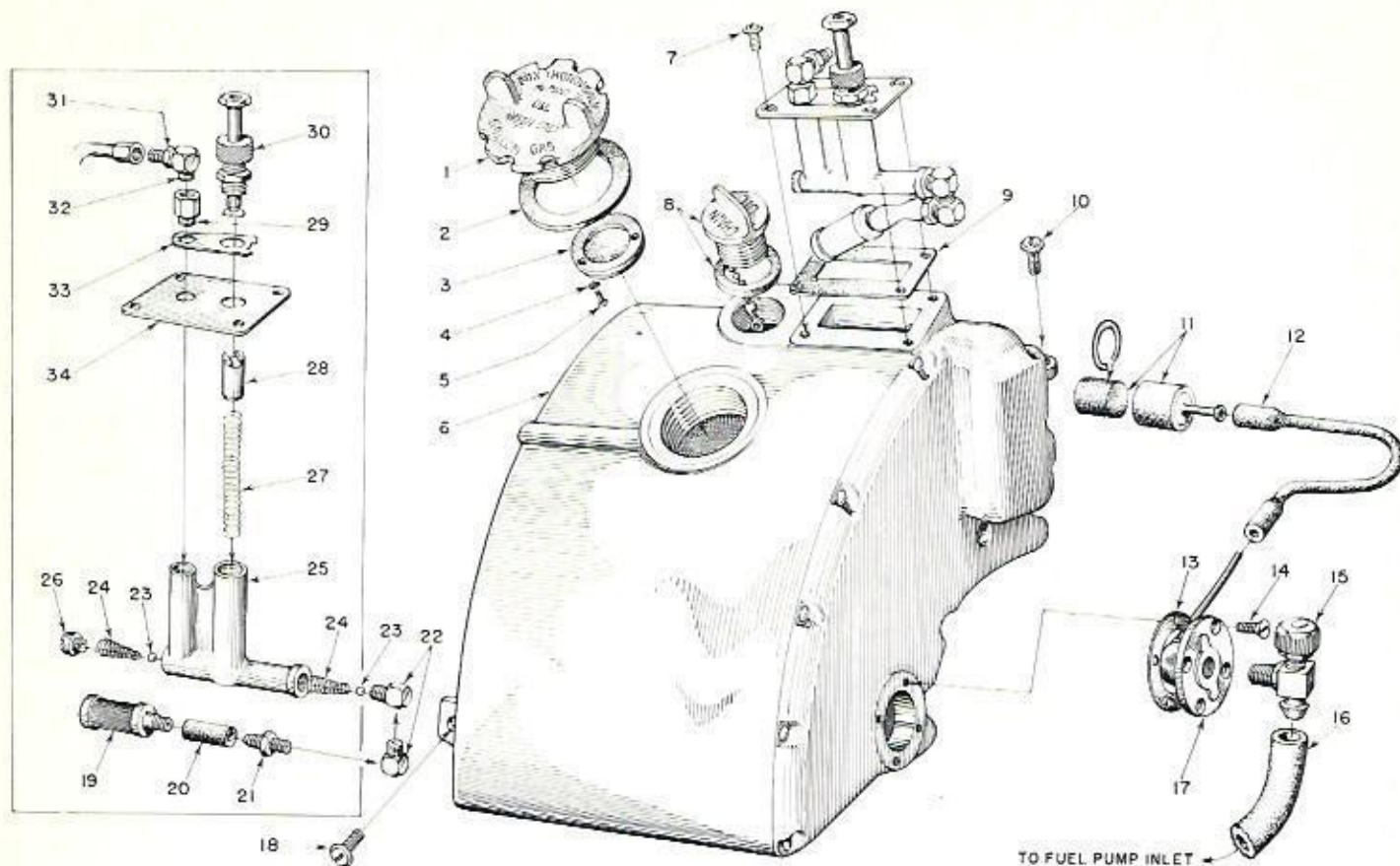
FIGURE 3—FUEL TANK PARTS
