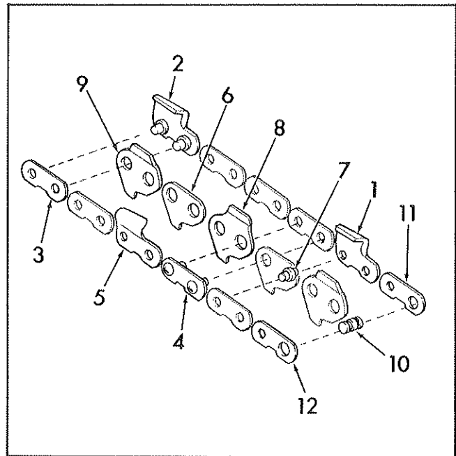
TYPE C3GH
