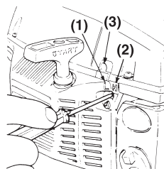
(1) L needle (2) H needle (3) Idle adjusting screw
