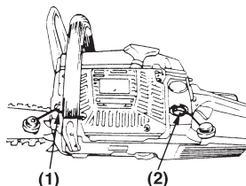
(1) Chain oil (2) Fuel
