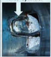
Pin Clip Lodged Into Cylinder
