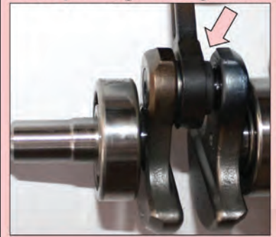
Over Speeding Bearing Failure
