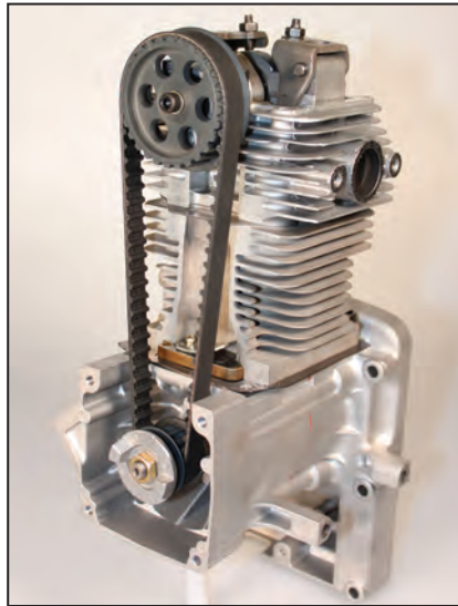
79.7cc Belt Drive Overhead Cam Engine
