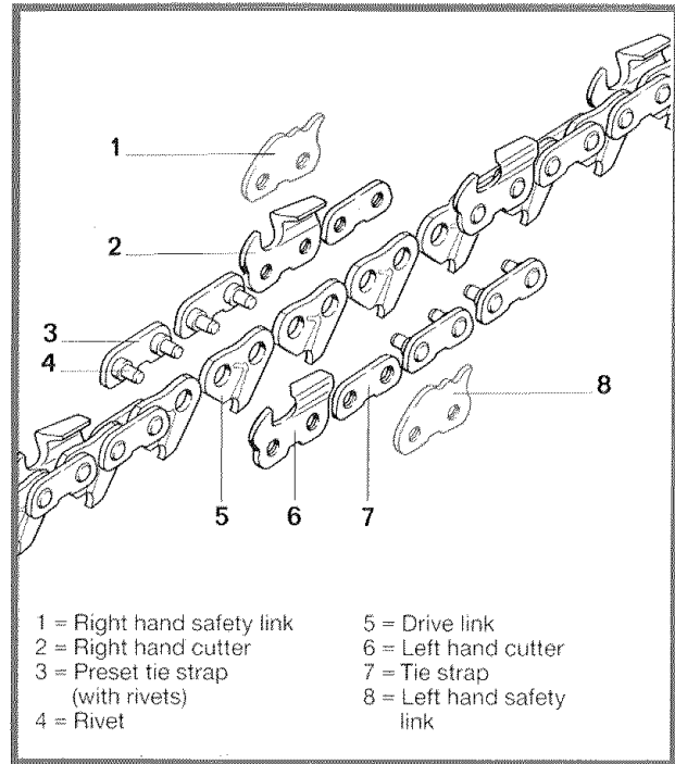
Top: Component parts of an Oilomatic chain Bottom: Measuring chain pitch "t"
