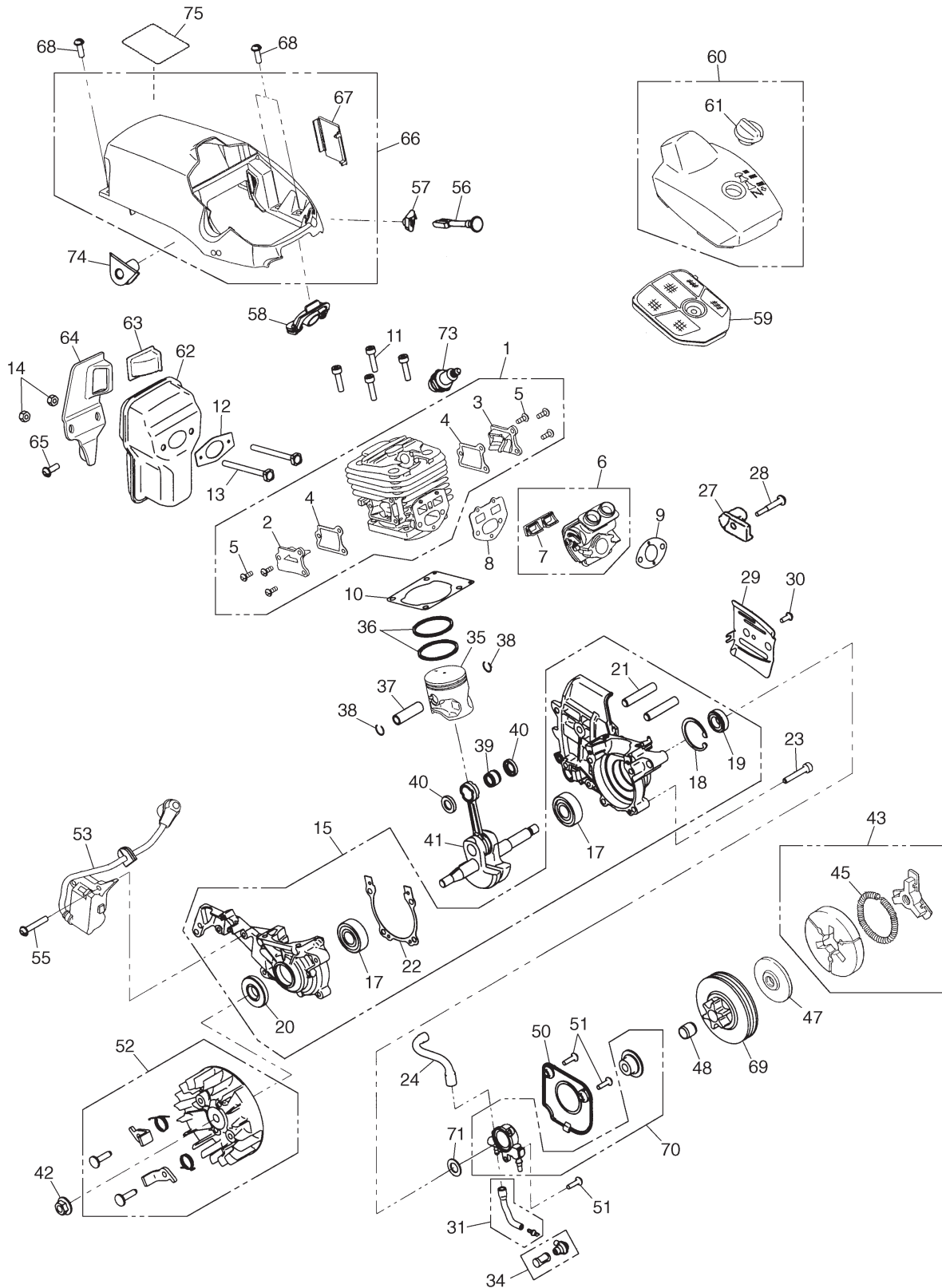
Fig.1 POWER UNIT (S/N 720401 and up)
