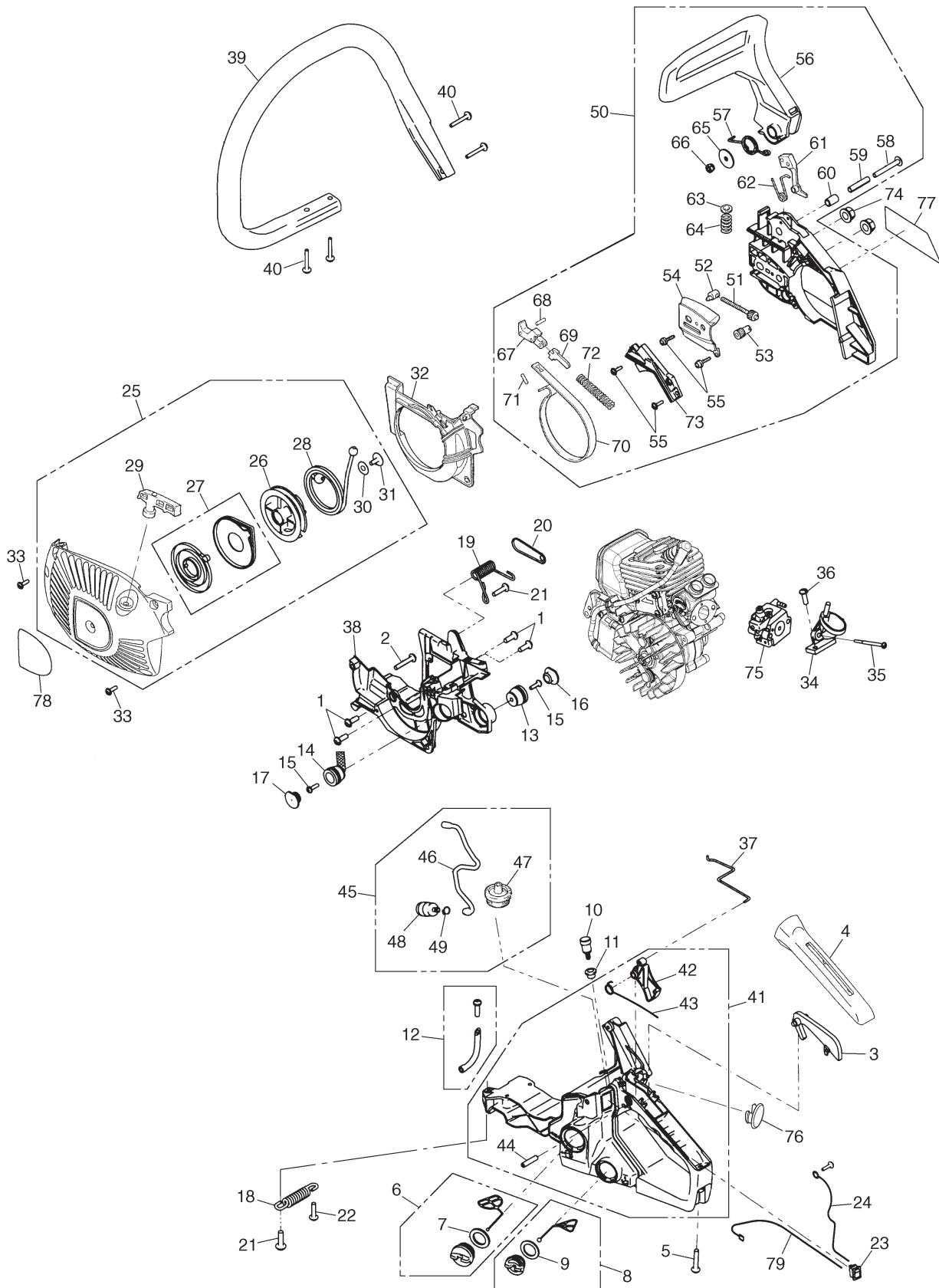
Fig.2 POWER UNIT (S/N 720401 and up)
