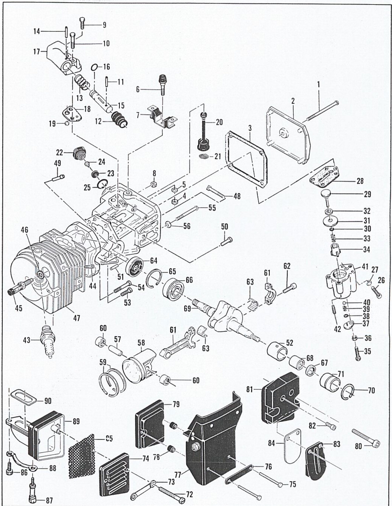
Figure 7. Powerhead and Oiler Assemblies
