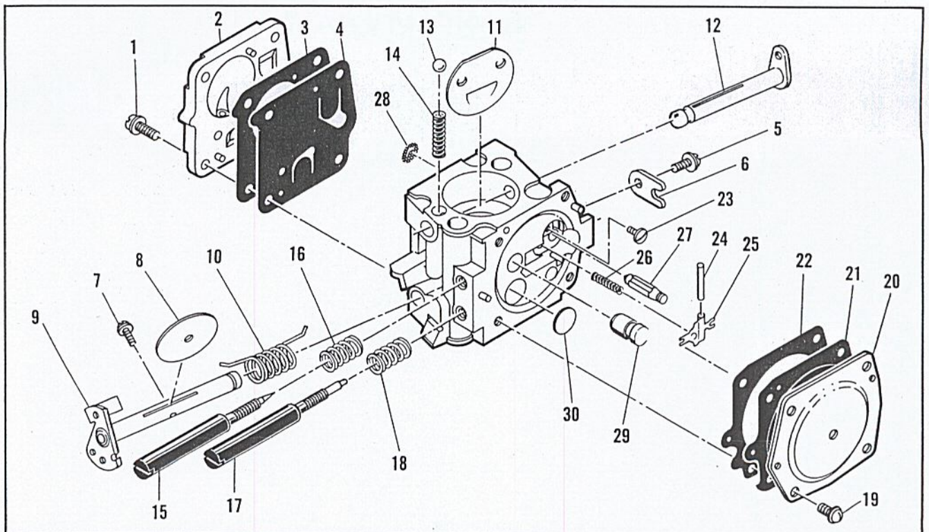
Figure 5. Carburetor Assembly
