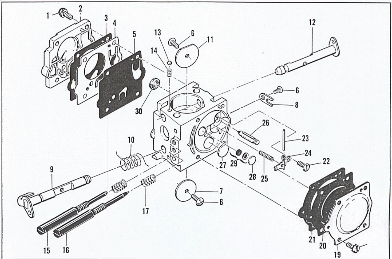
Figure 4. Carburetor Assembly
