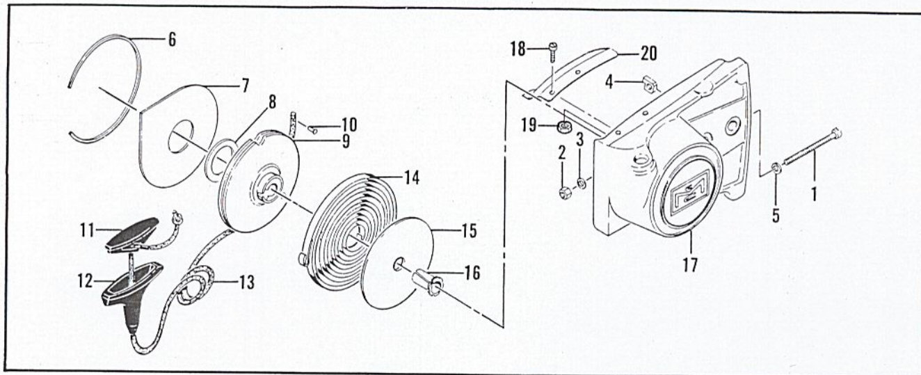
Figure 2. Clutch Guard and Starter Assembly
