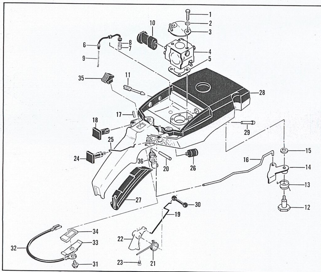
Figure 3. Fuel Tank Assembly
