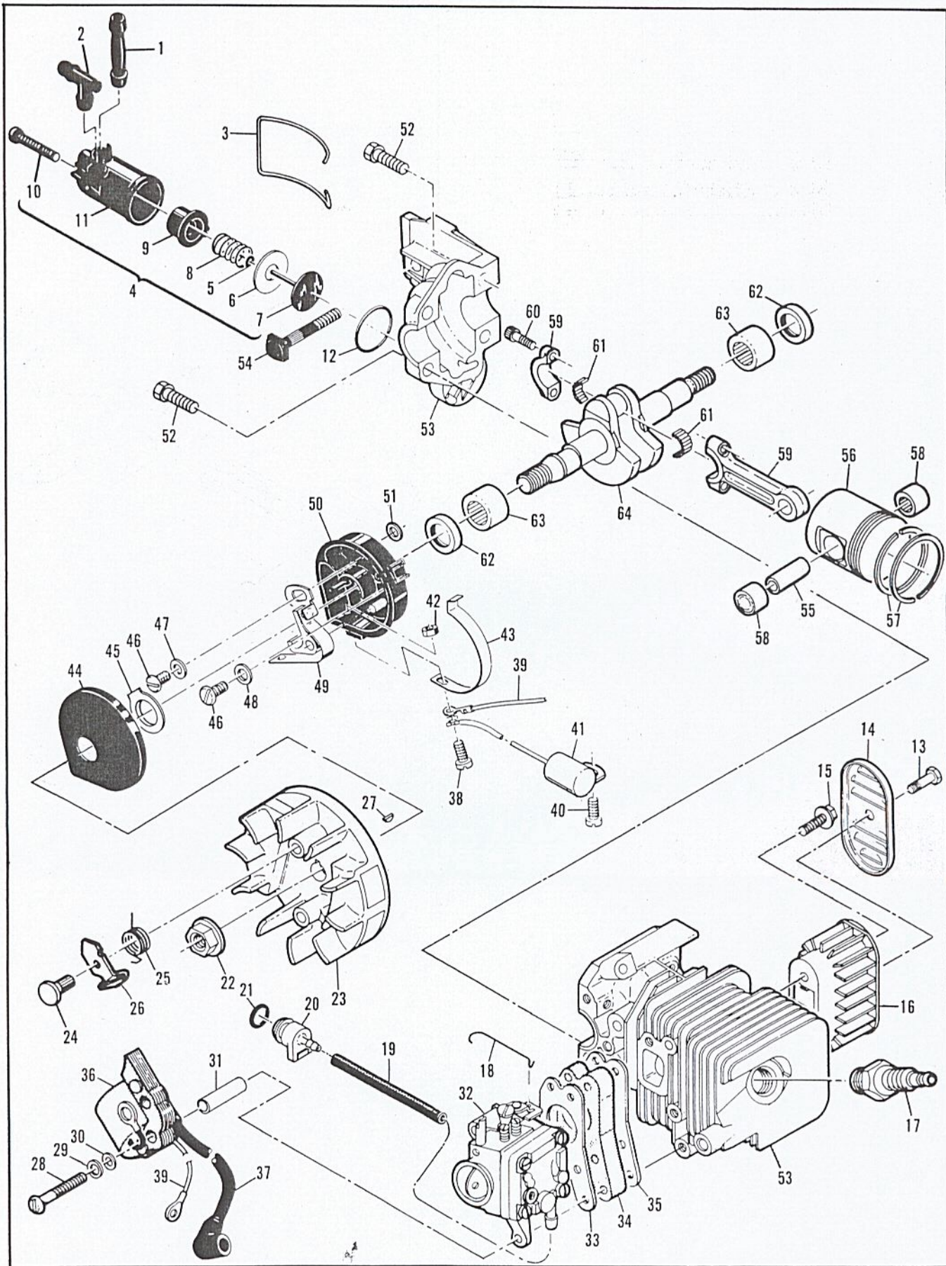
Figure 4. Powerhead Assembly
