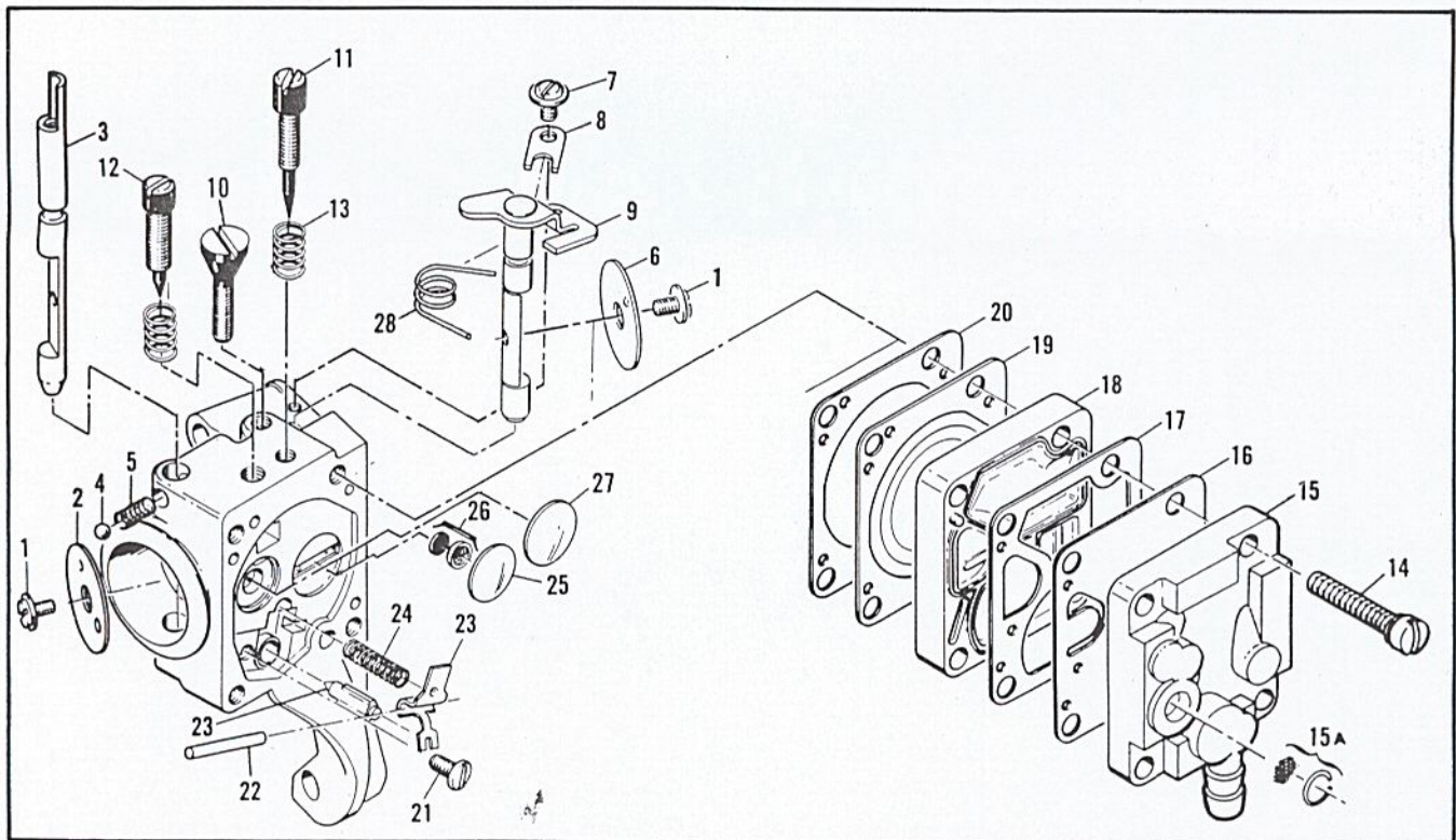
Figure 3. Carburetor Assembly
