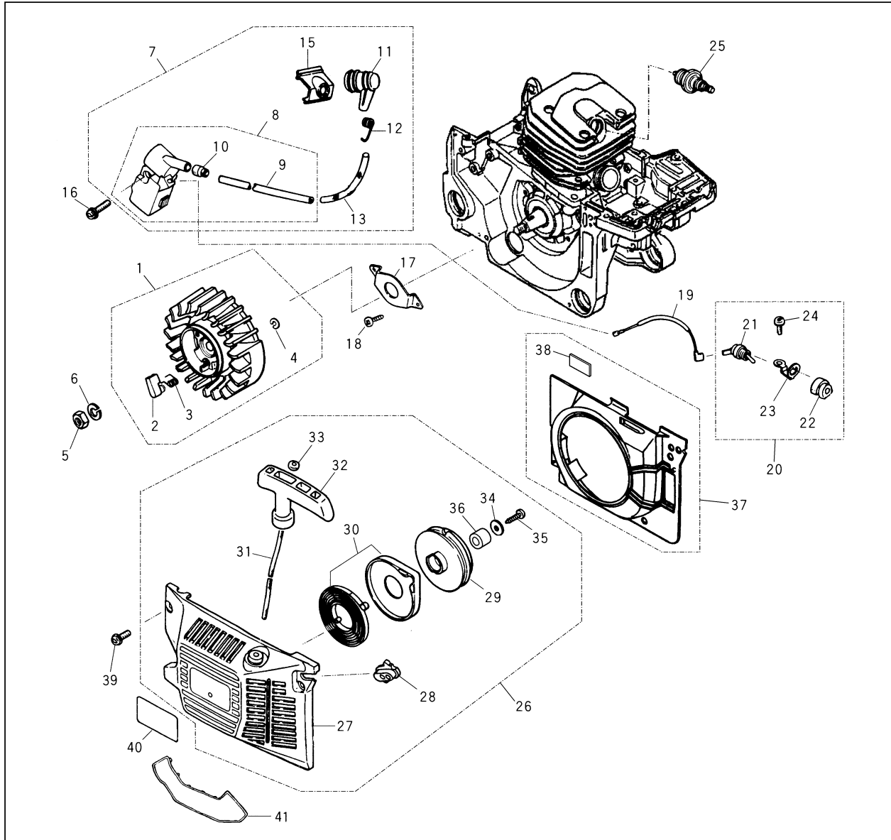
Fig.2 IGNITION SYSTEM, STARTER
