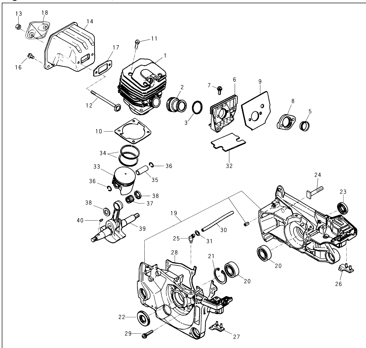
Fig.1 ENGINE BLOCK, MUFFLER
