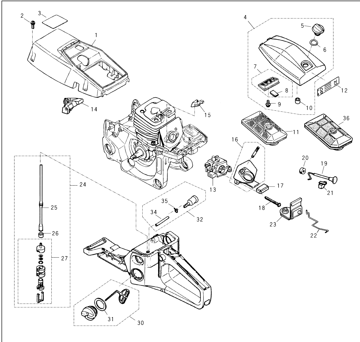
Fig.4 FUEL SUPPLY SYSTEM
