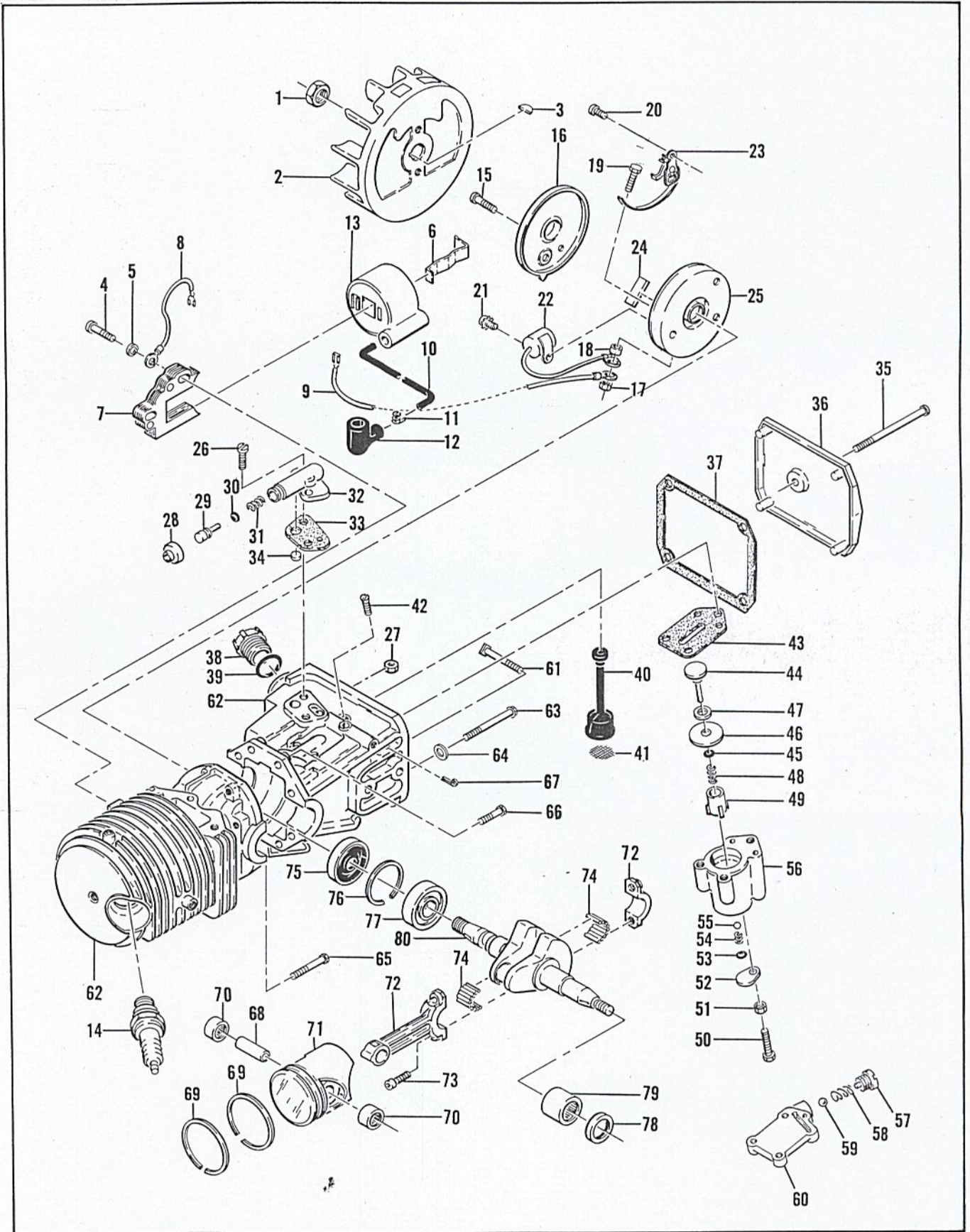
Figure 5. Powerhead Assembly
