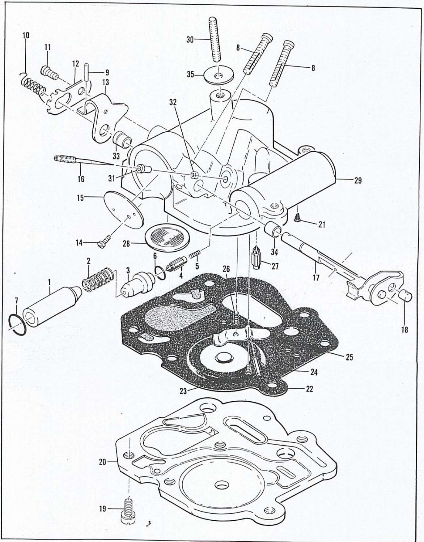
Figure 4. Carburetor Assembly
