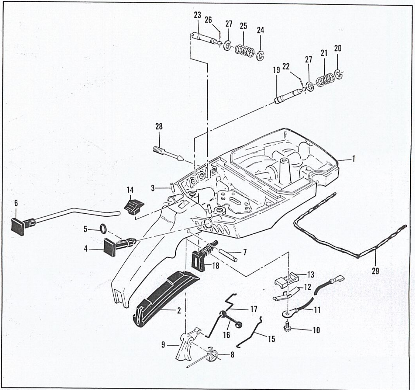
Figure 3. Fuel Tank Assembly
