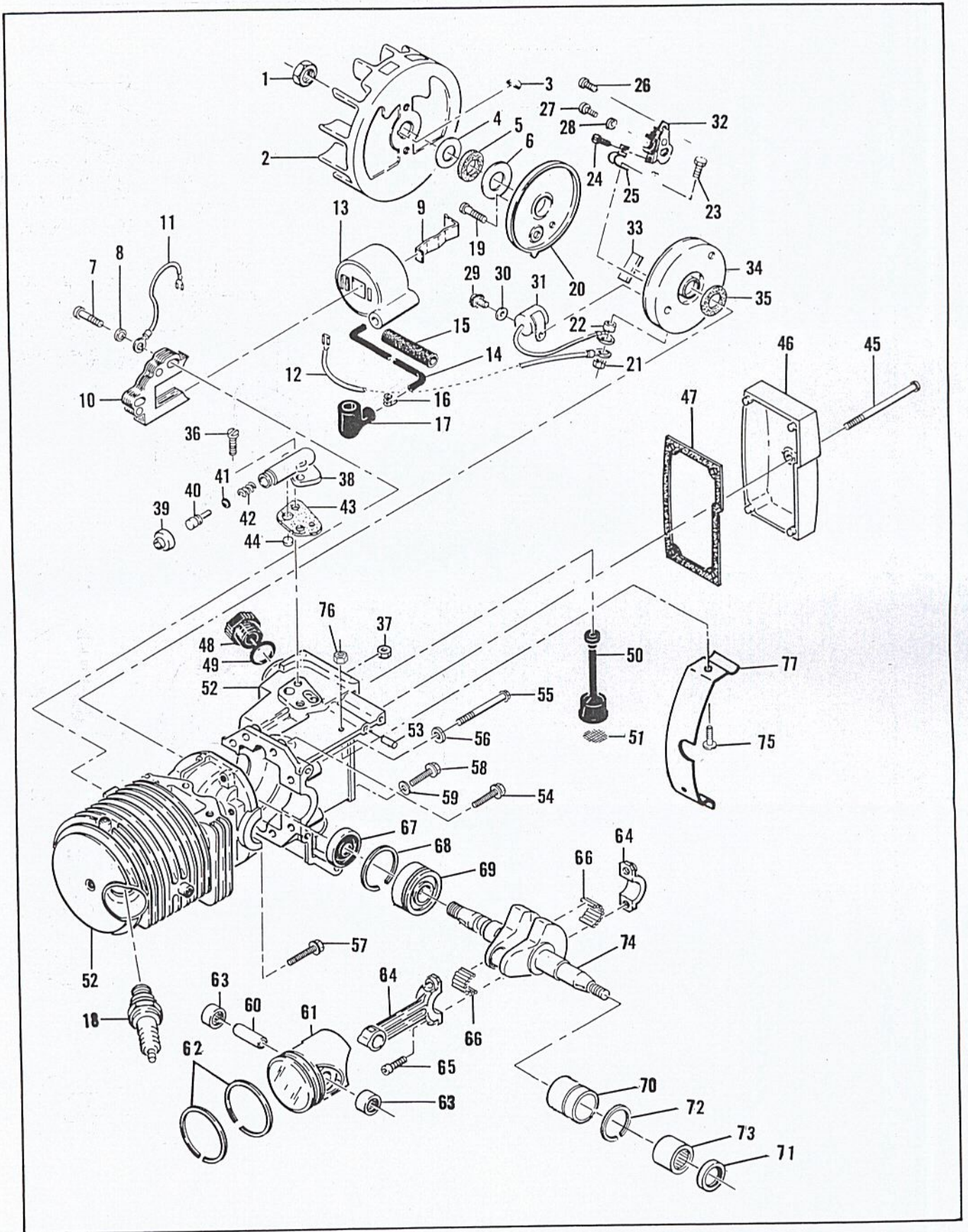
Figure 7. Powerhead Assembly
