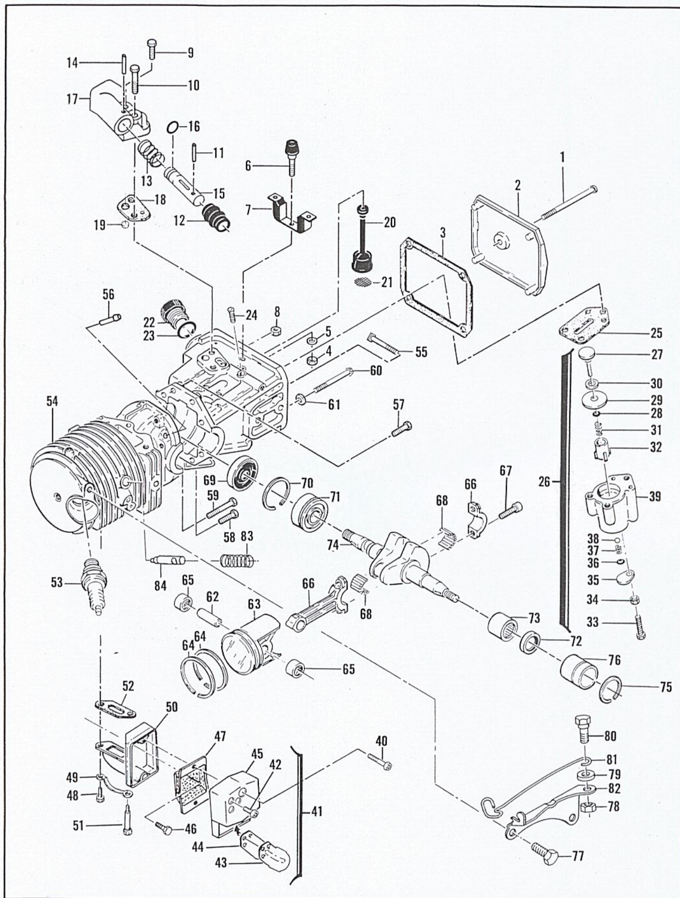
Figure 6. Powerhead and Oiler Assemblies
