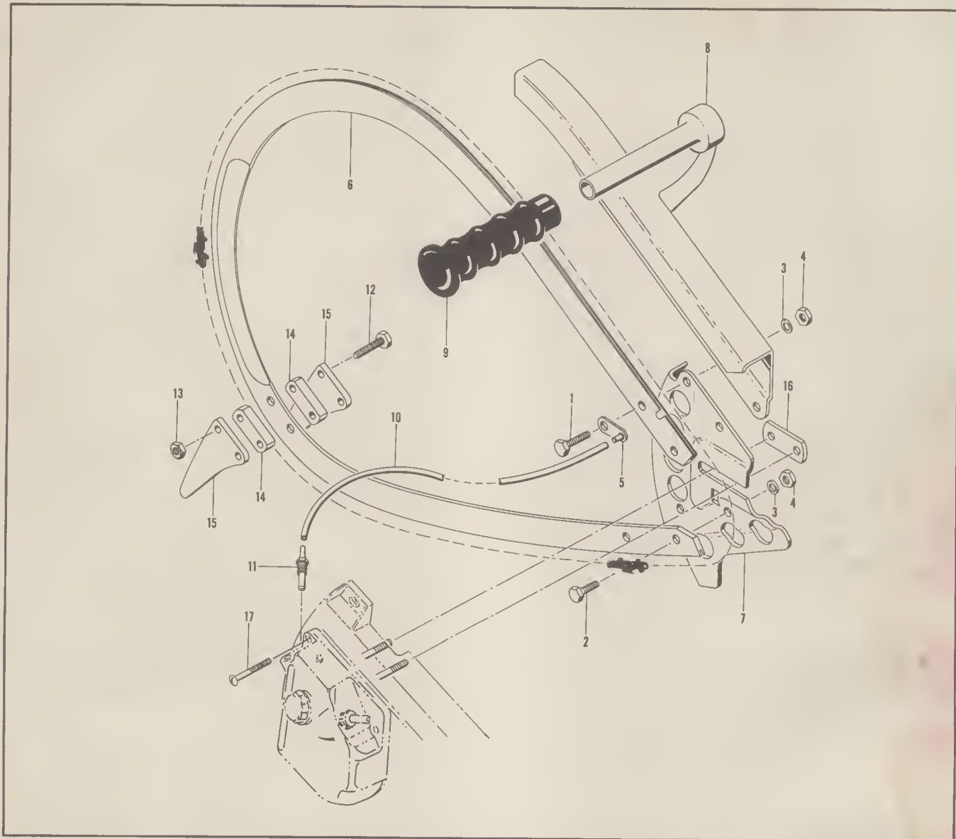
FIGURE 7. PLUNGE BOW SAW ASSEMBLY
