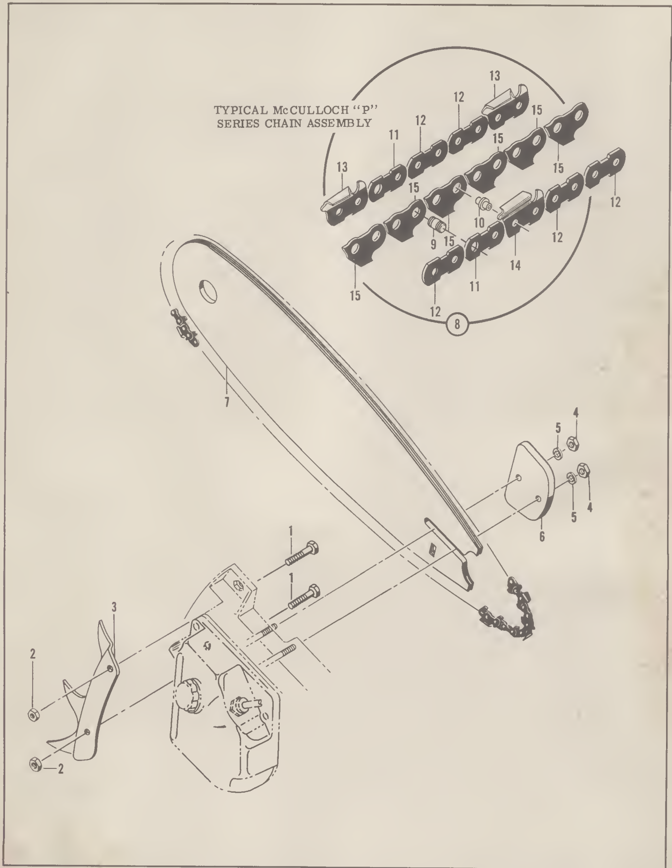
Figure 6. Saw Blade, Spike, Chain and Lockplate
