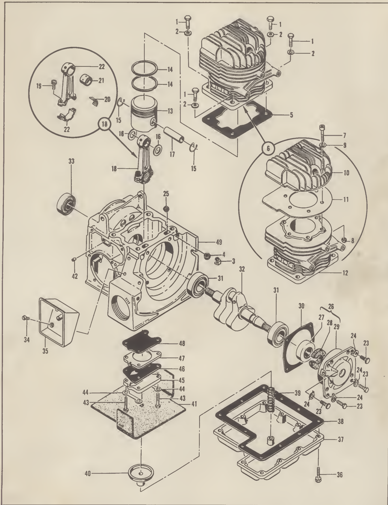
Figure 5. Crankcase, Crankshaft, Cylinder and Piston
