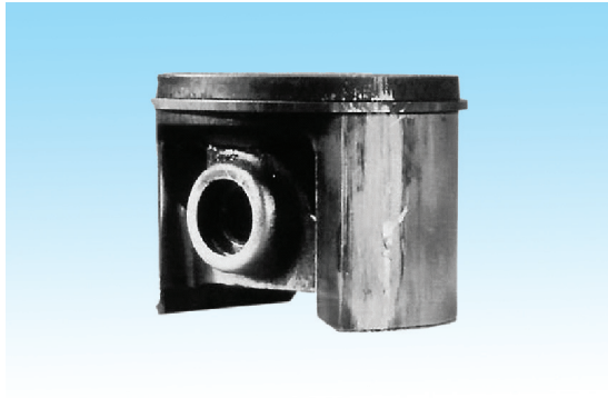
Small to medium scoring within the exhaust port area
