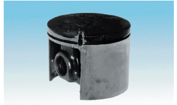
The locating pin for the piston ring has been pushed up through the top of piston
